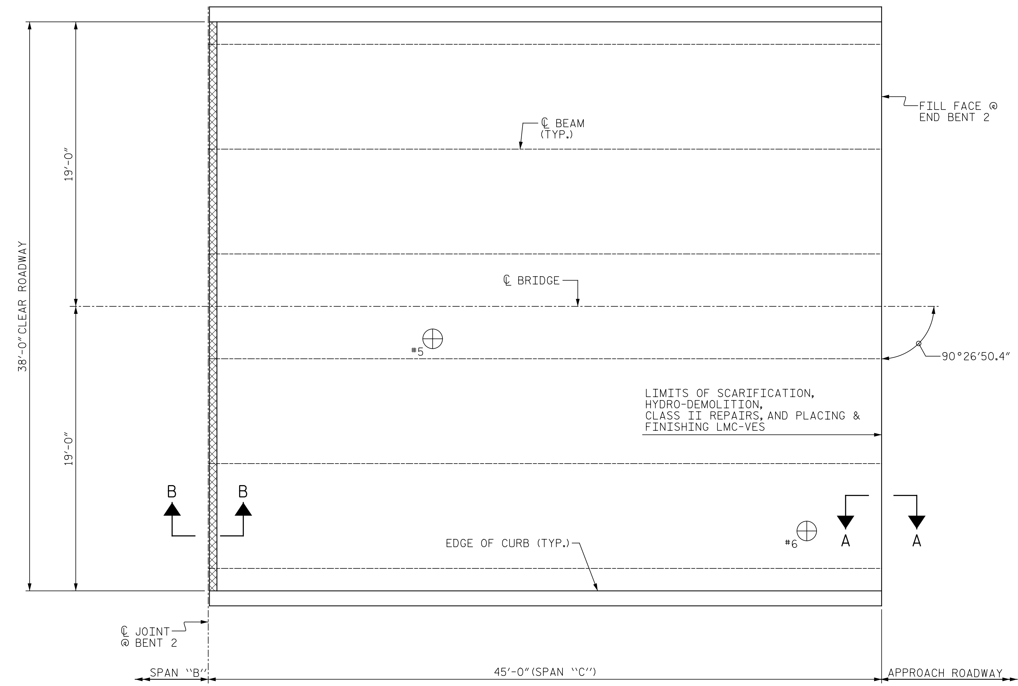
PLAN OF SPAN "C" (SEE SHEET NO. S-131 FOR SECTIONS A-A AND B-B)
