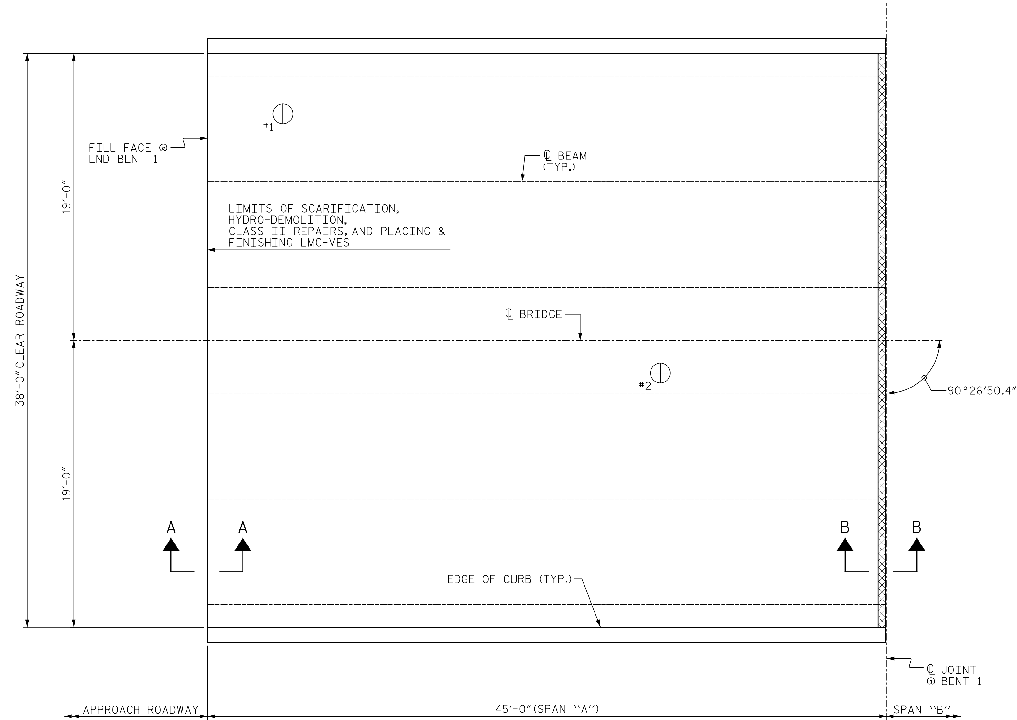
PLAN OF SPAN "A" (SEE SHEET NO. S-131 FOR SECTIONS A-A AND B-B)
