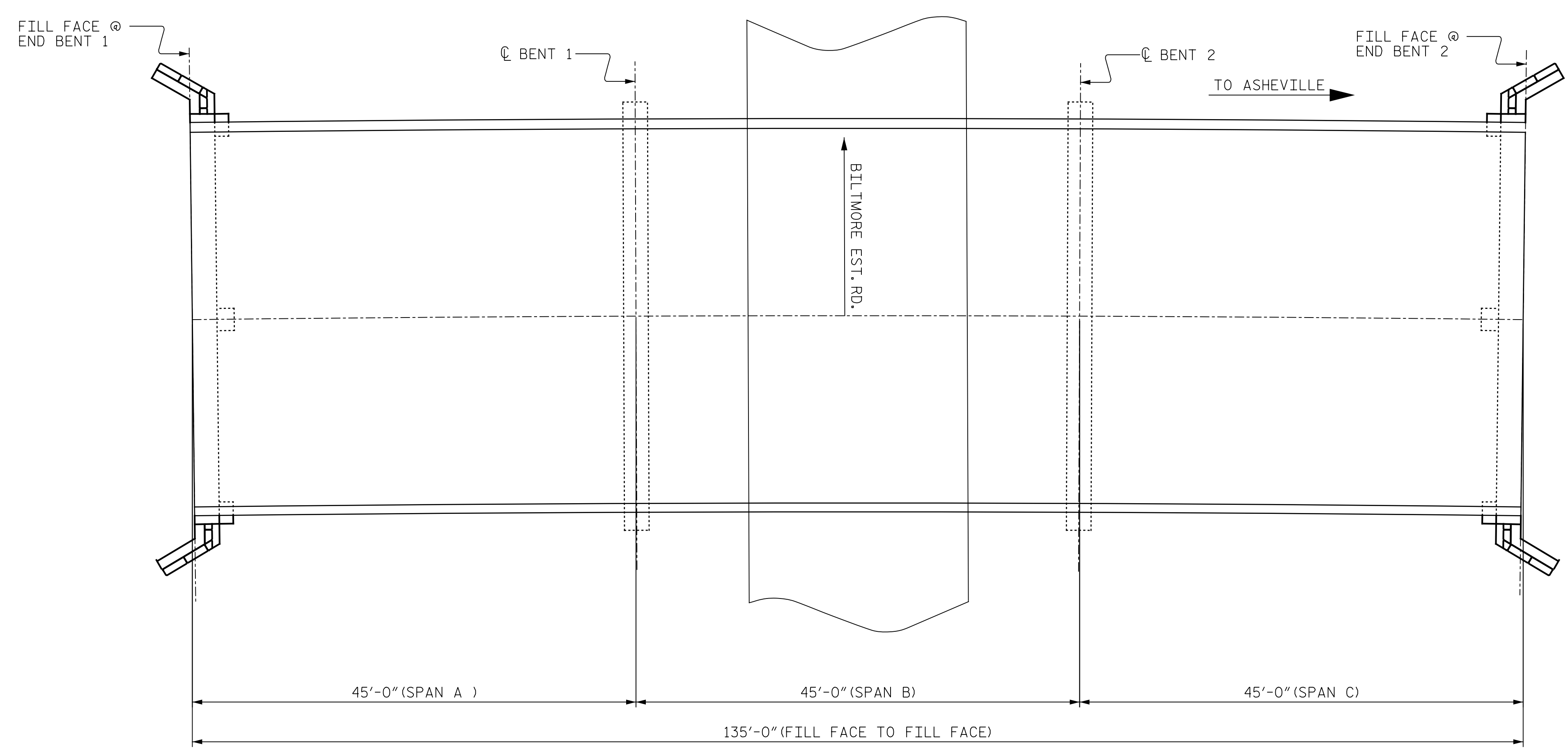
PLAN (PILES NOT SHOWN FOR CLARITY)
