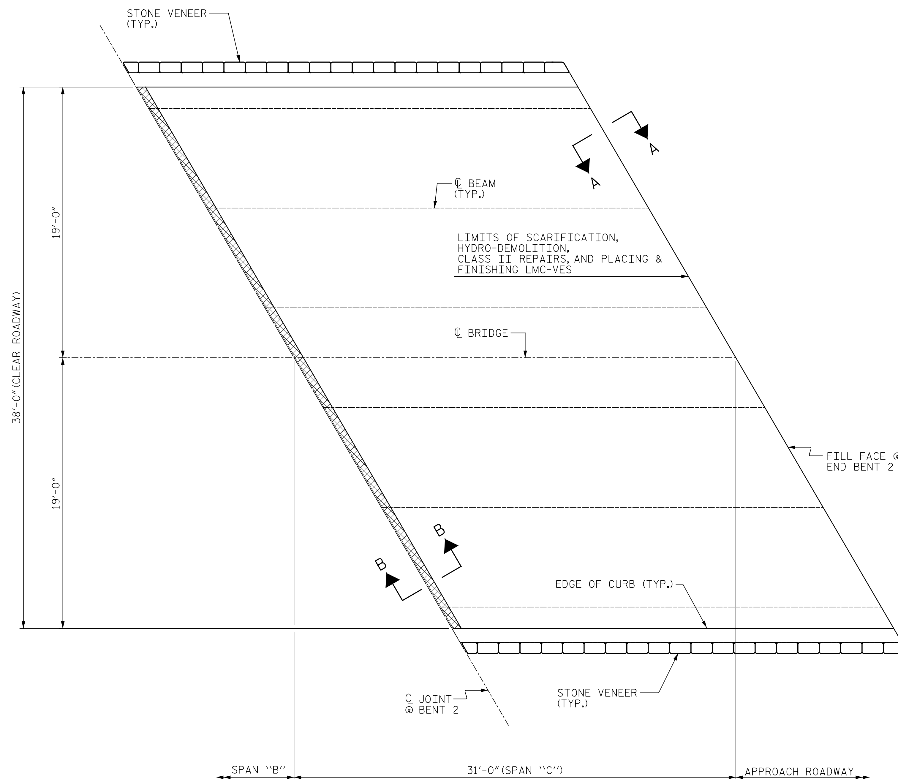
PLAN OF SPAN "C" (SEE SHEET NO. S-112 FOR SECTIONS A-A AND B-B)
