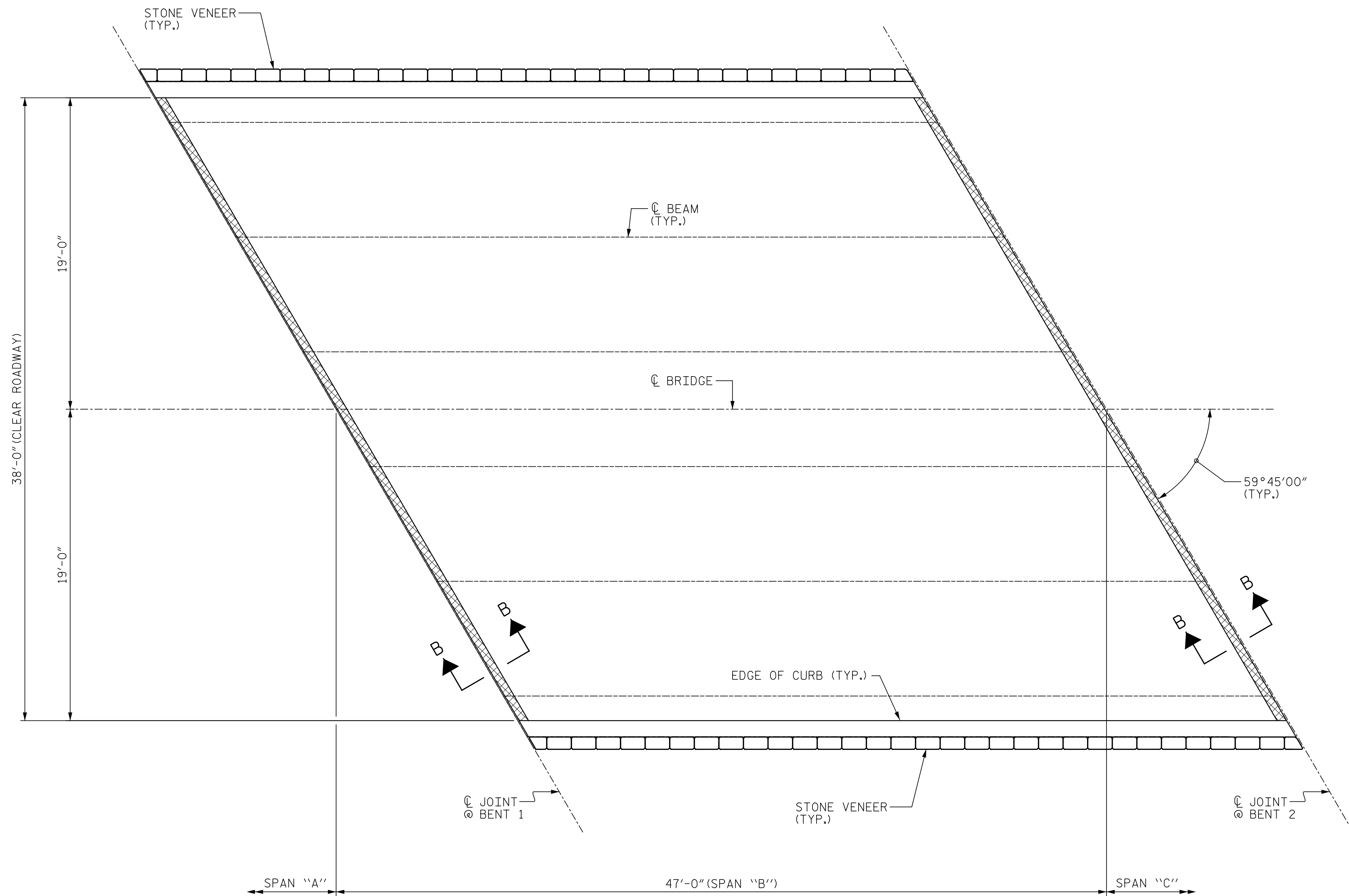
PLAN OF SPAN "B" (SEE SHEET NO. S-112 FOR SECTION B-B)
