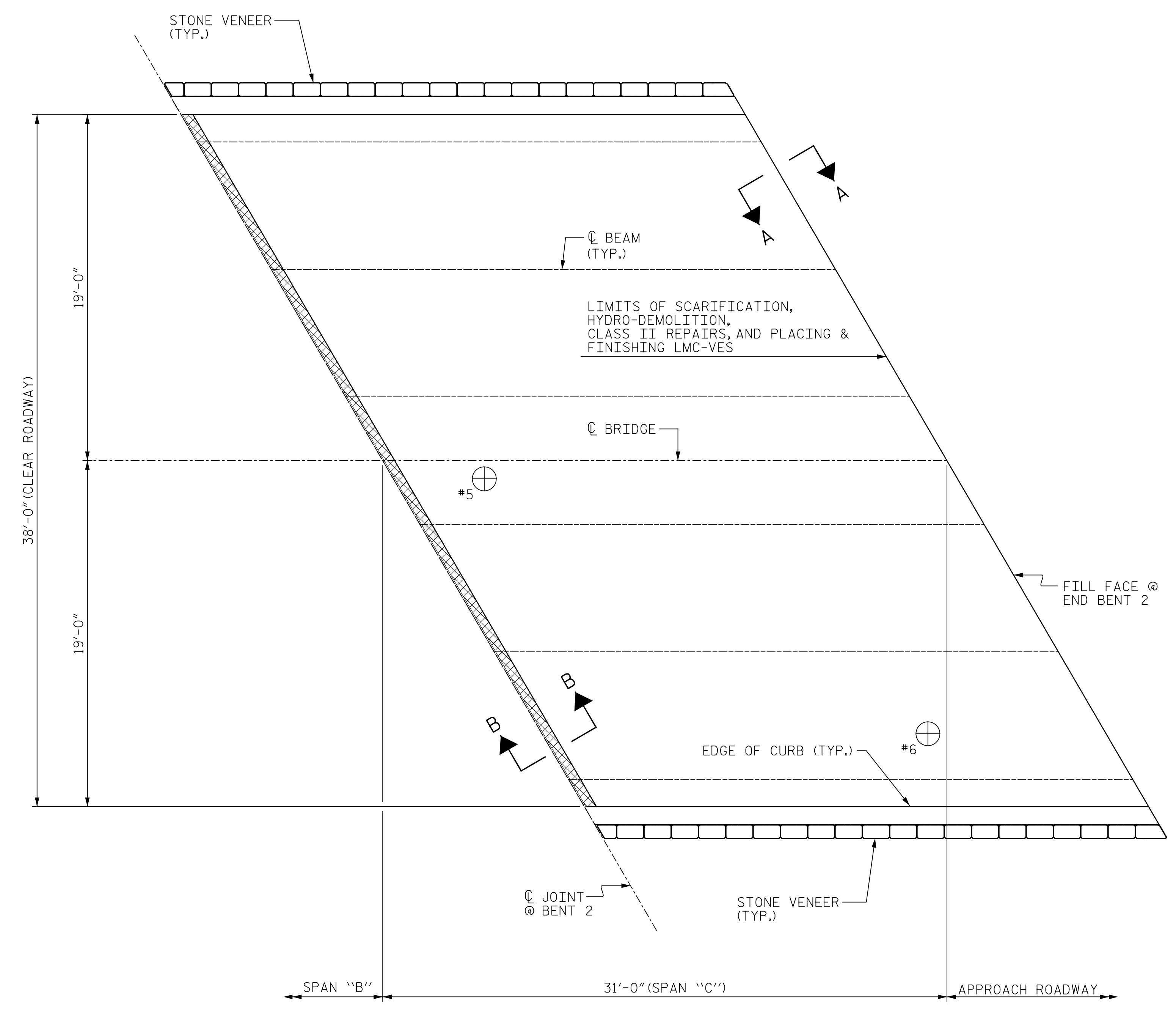
PLAN OF SPAN "C" (SEE SHEET NO. S-93 FOR SECTIONS A-A AND B-B)
