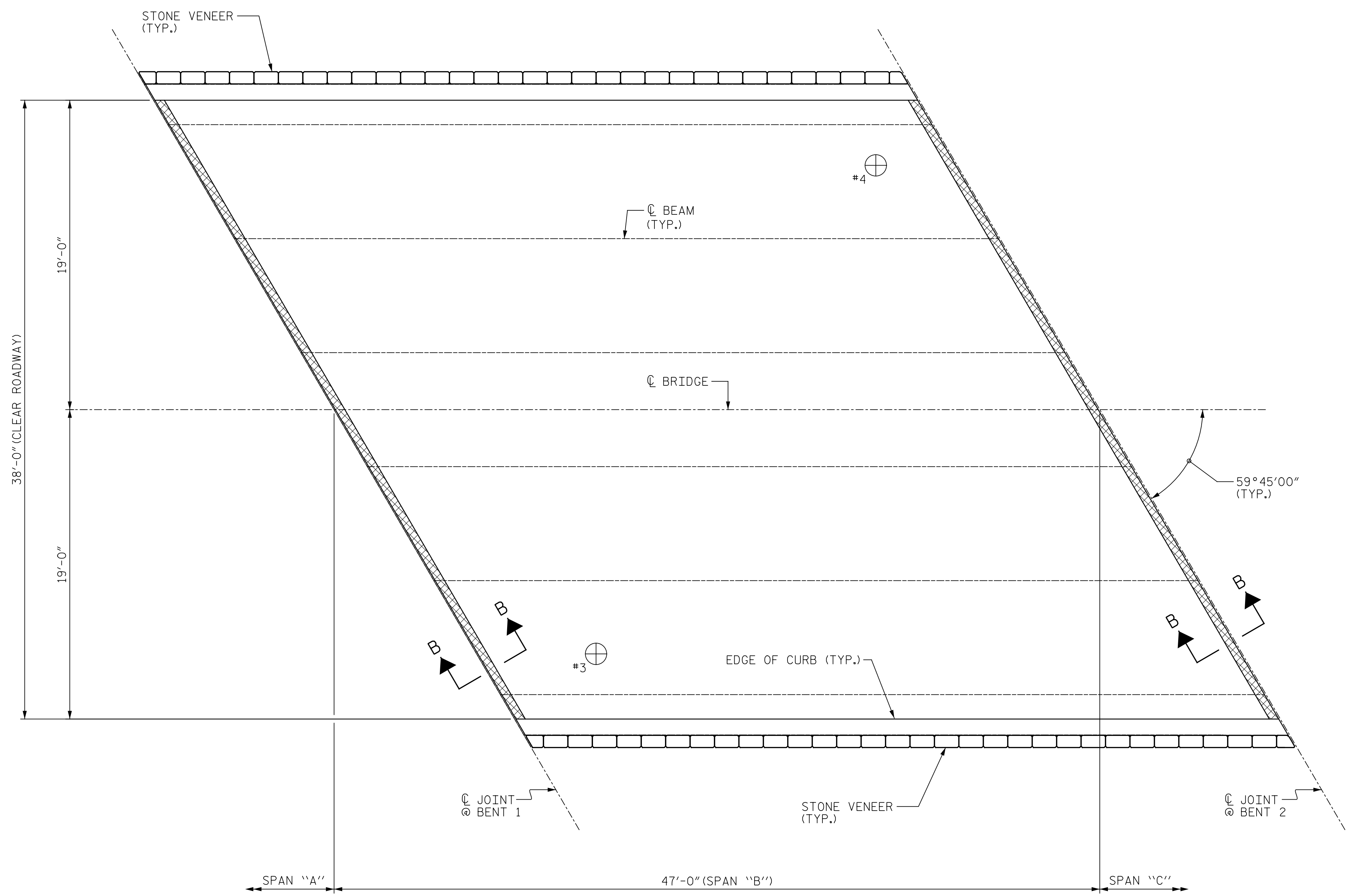
PLAN OF SPAN "B" (SEE SHEET NO. S-93 FOR SECTION B-B)
