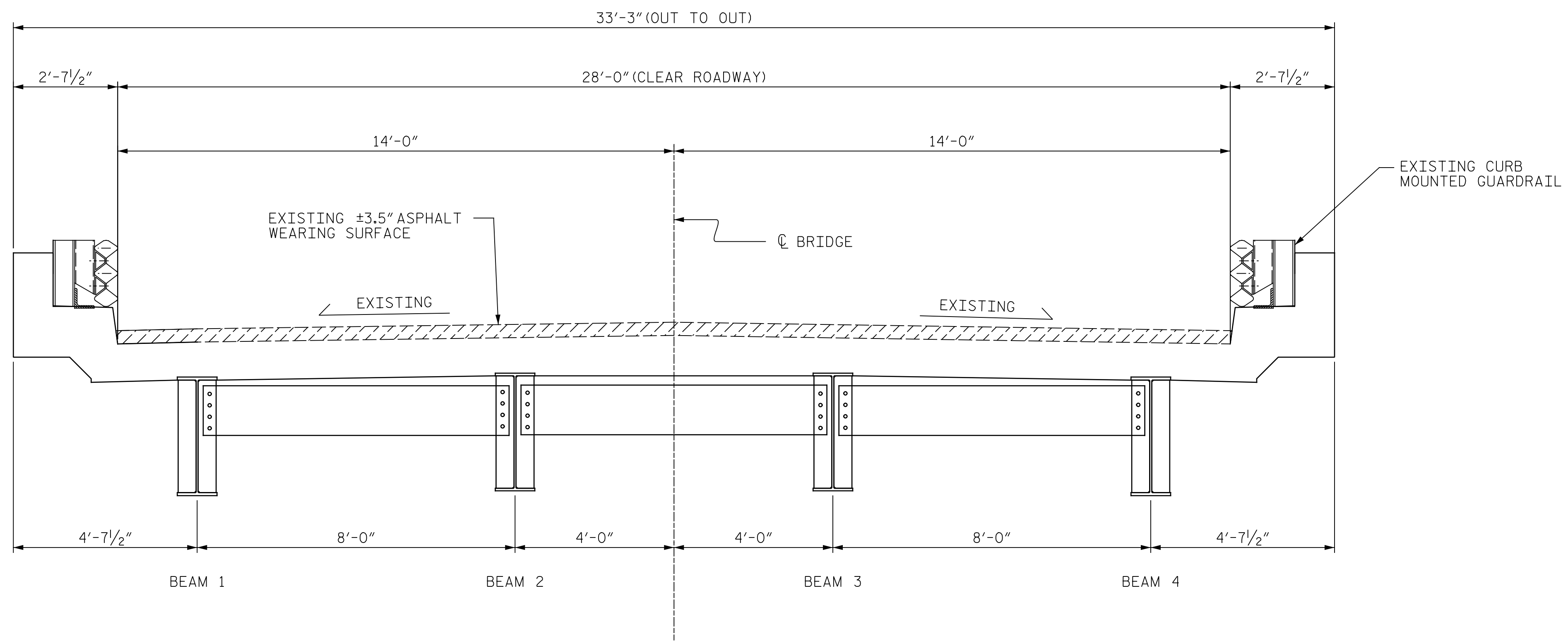
TYPICAL SECTION (EXISTING)
