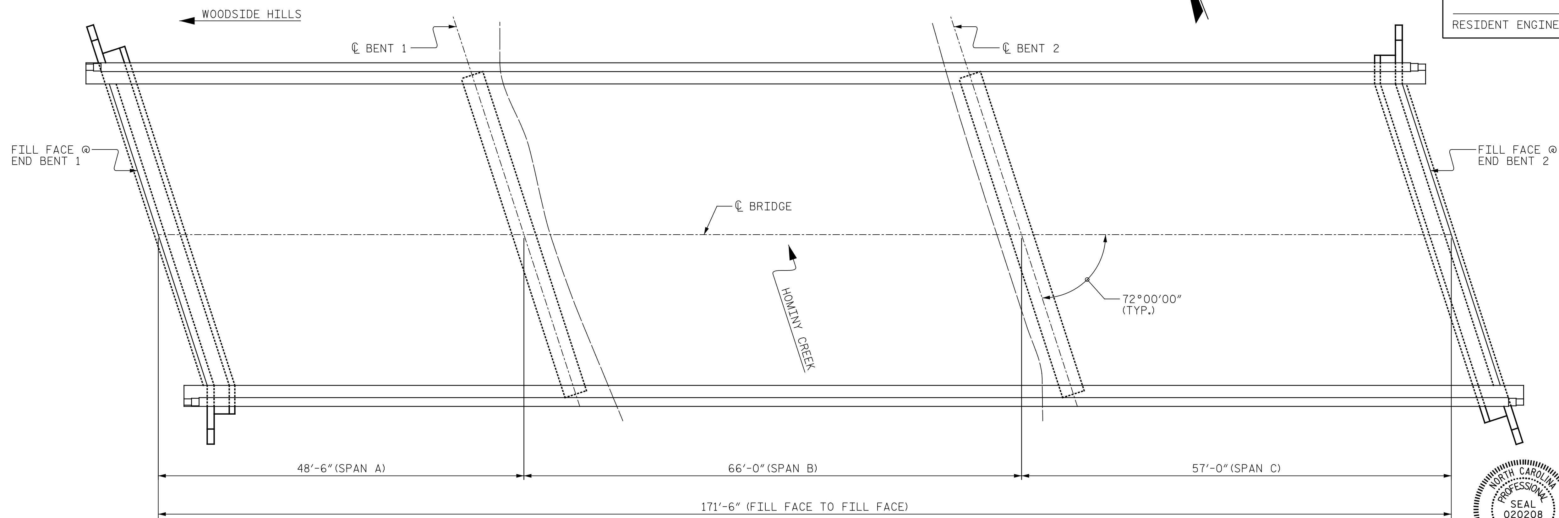
PLAN (PILES NOT SHOWN FOR CLARITY)
