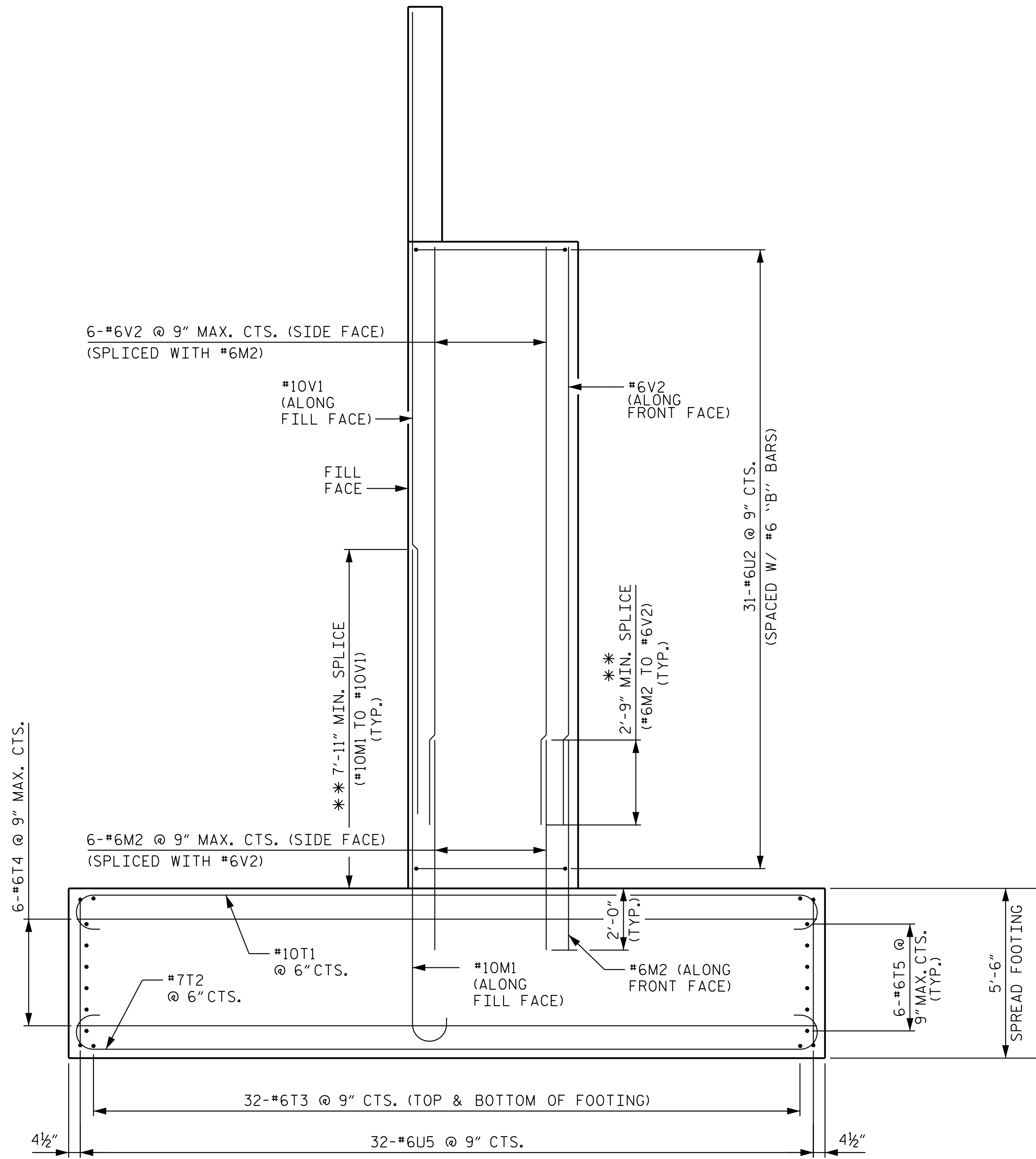
VIEW X-X
