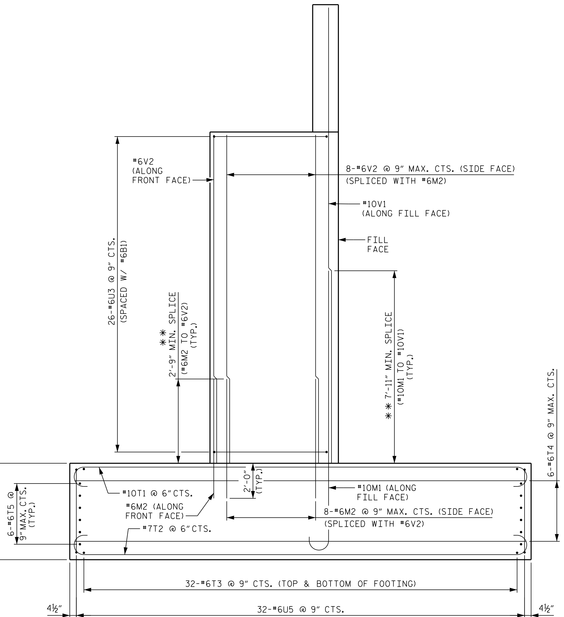
VIEW Y-Y
