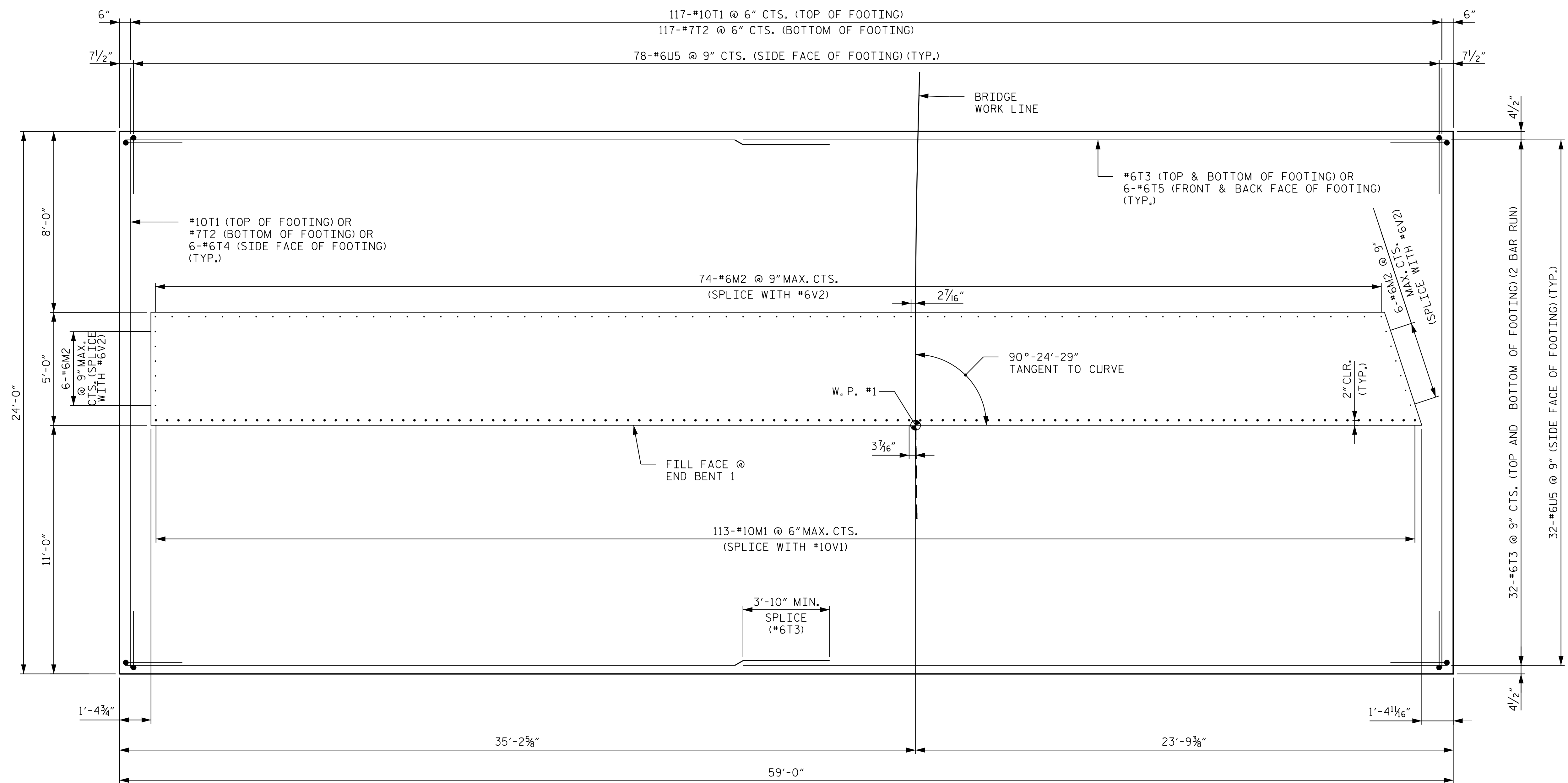
FOOTING PLAN
