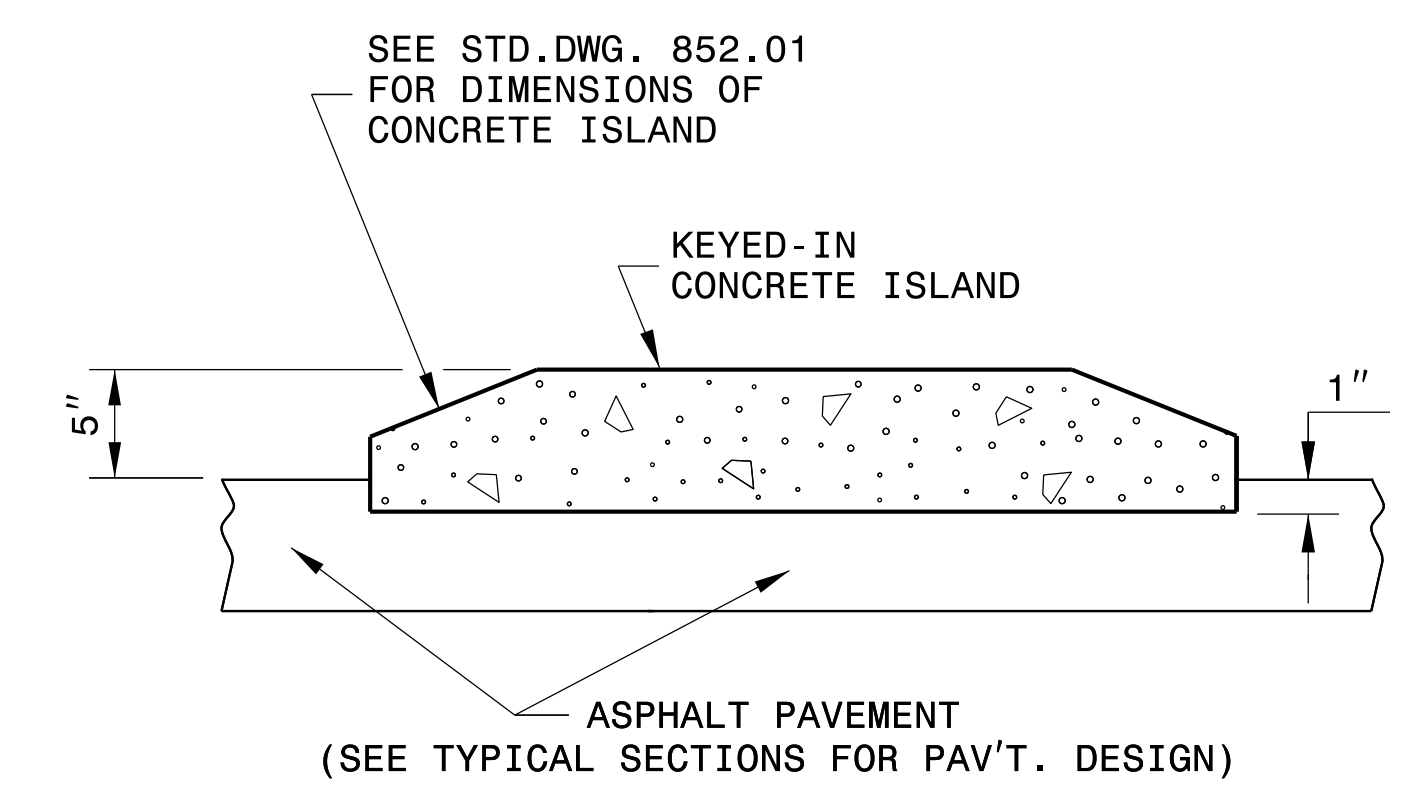
SECTION C-C
