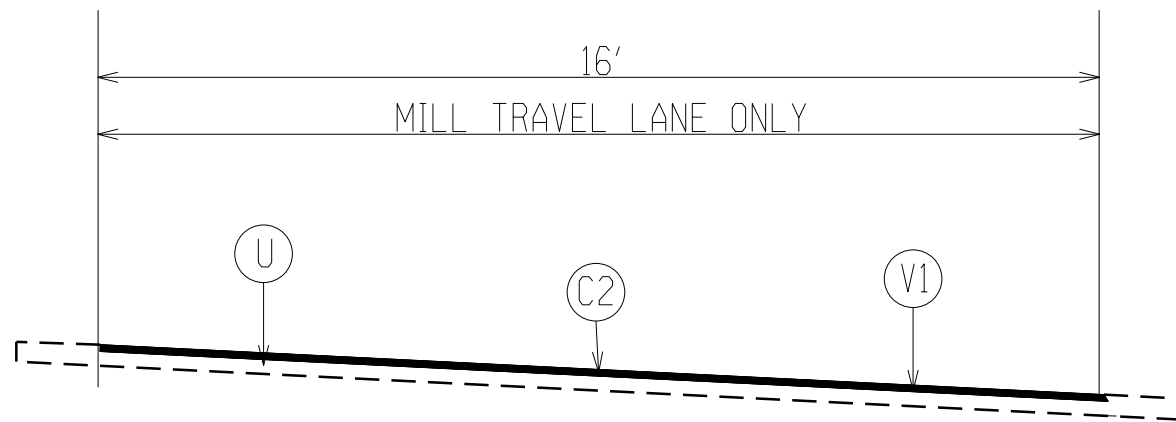
TYPICAL SECTION 2
