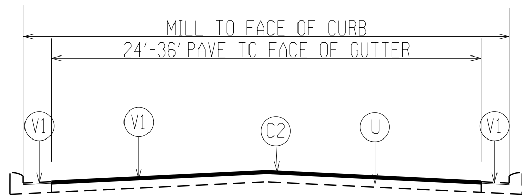
TYPICAL SECTION 3
