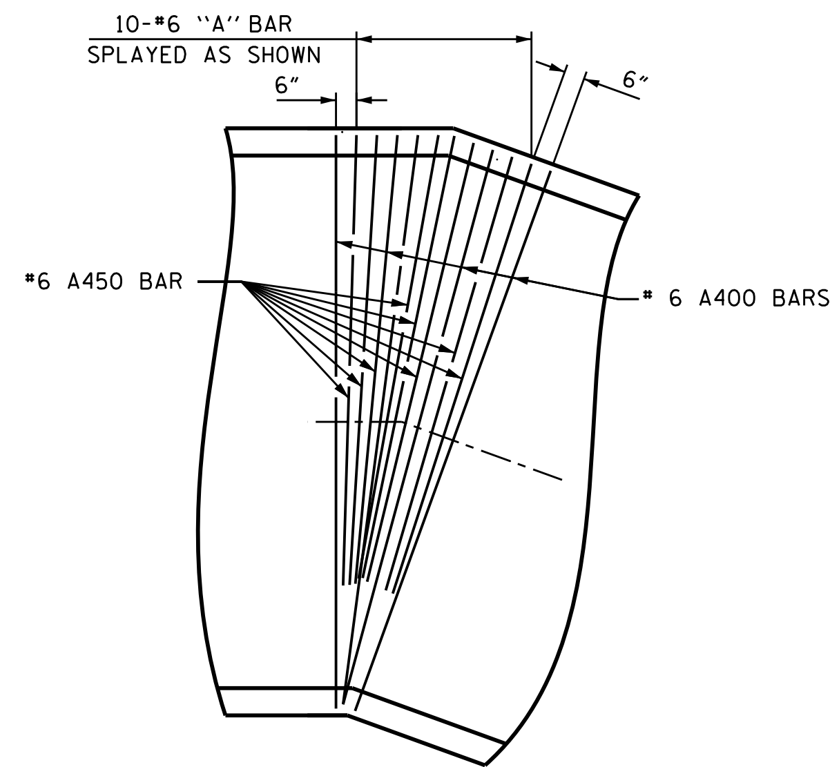
DETAIL A
