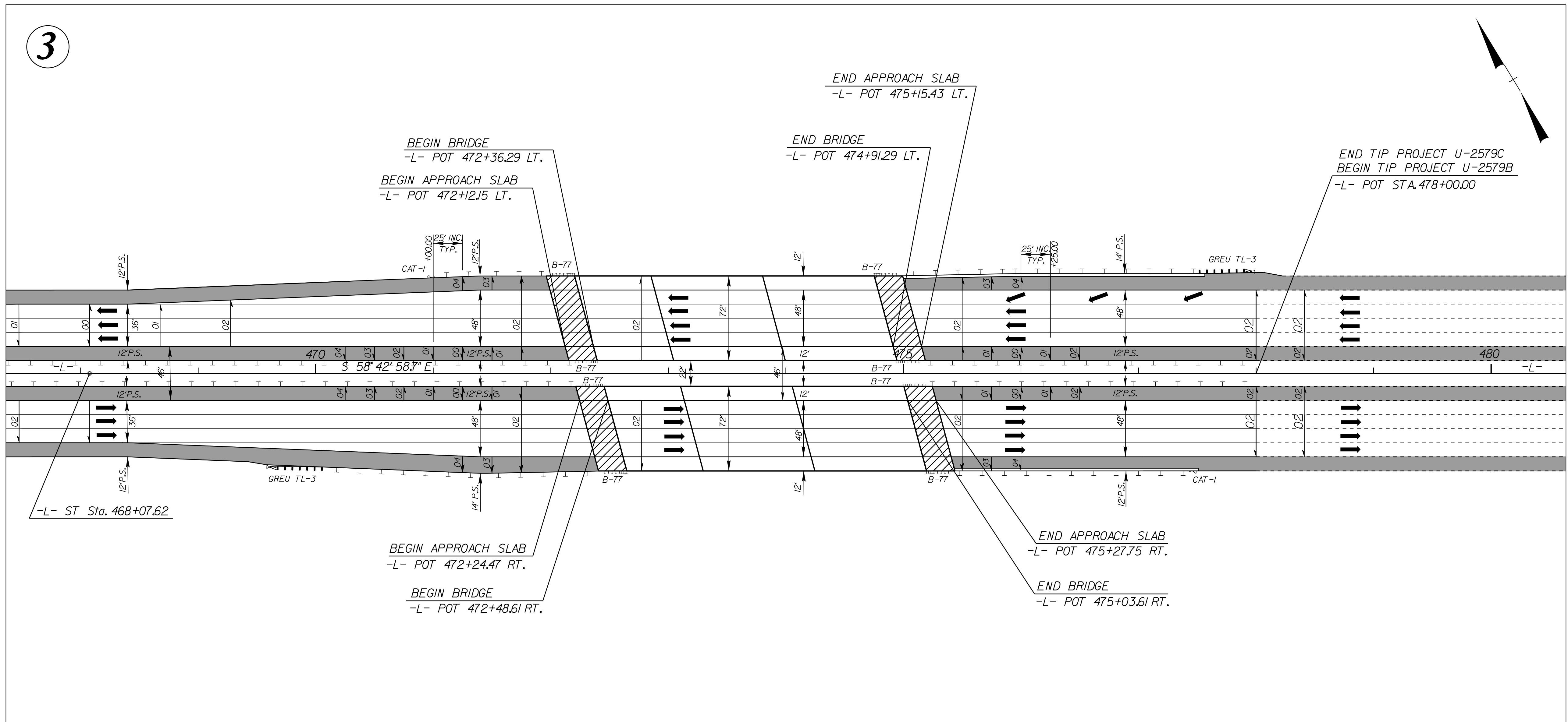
DETAIL SHOWING PAVEMENT & BRIDGE RELATIONSHIP FOR -L- (DUAL BRIDGES) OVER LOWERY MILL CREEK
