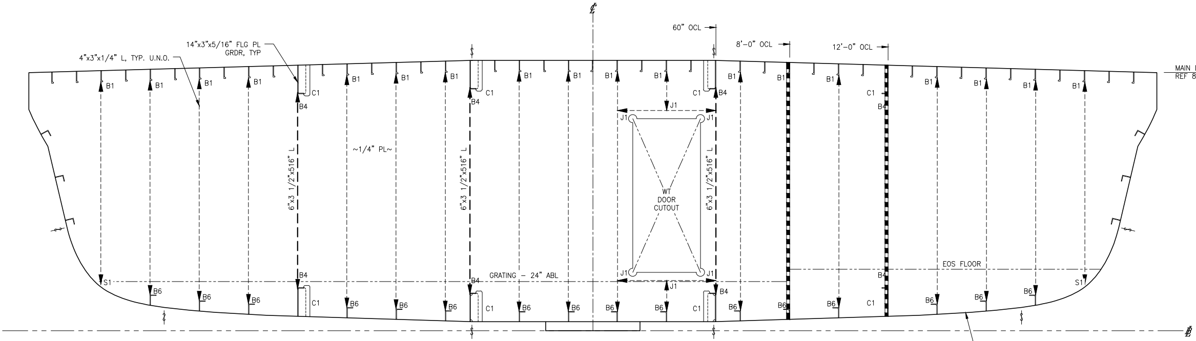
SECTION 2-4A FRAME 14, 'B' END LOOKING FWD
