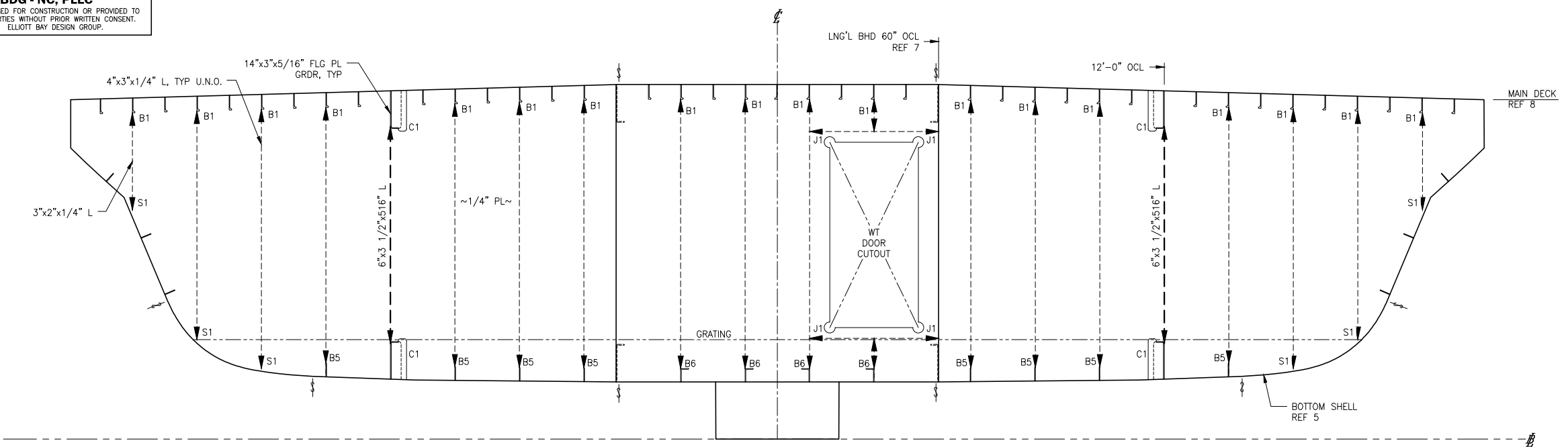
SECTION 2-4C FRAME 24, 'B' END LOOKING FWD
