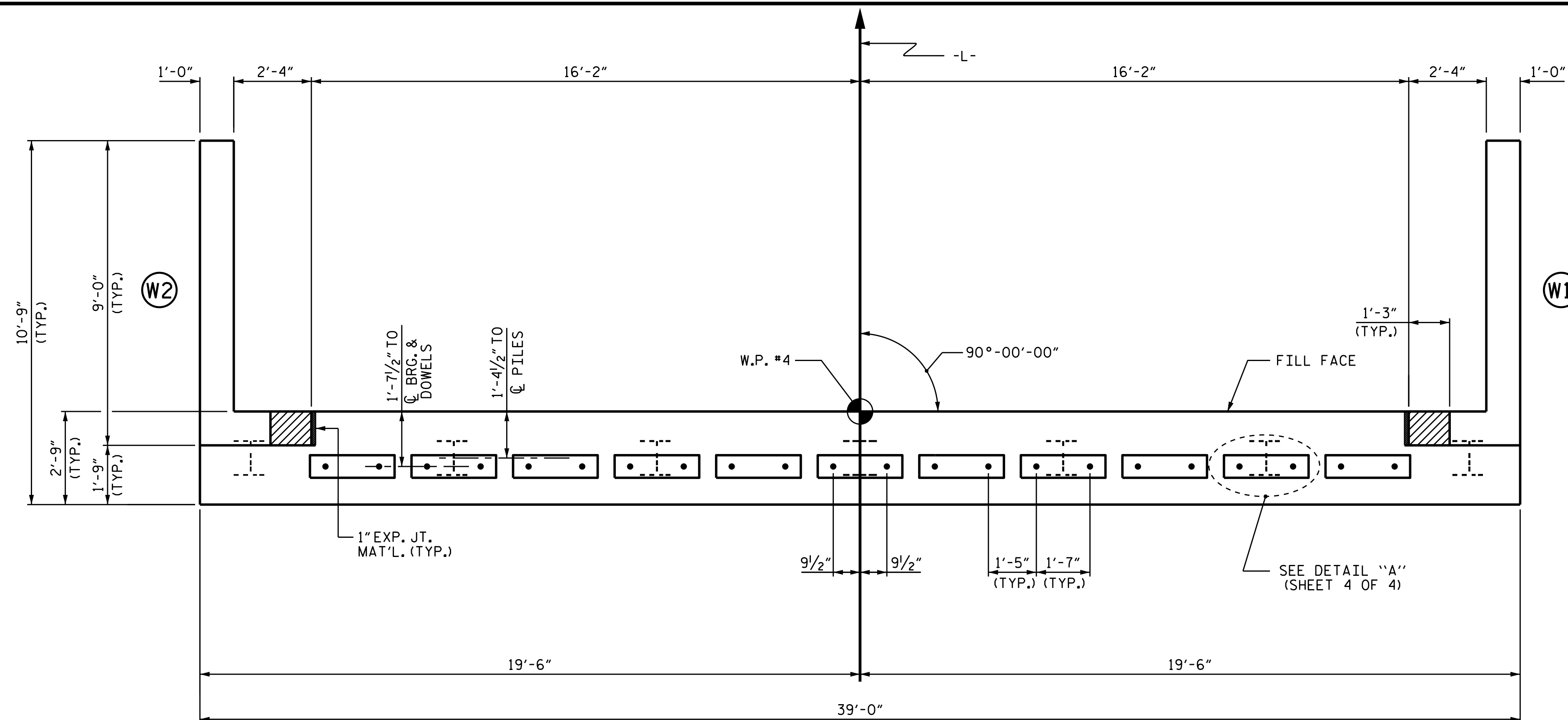
PLAN
