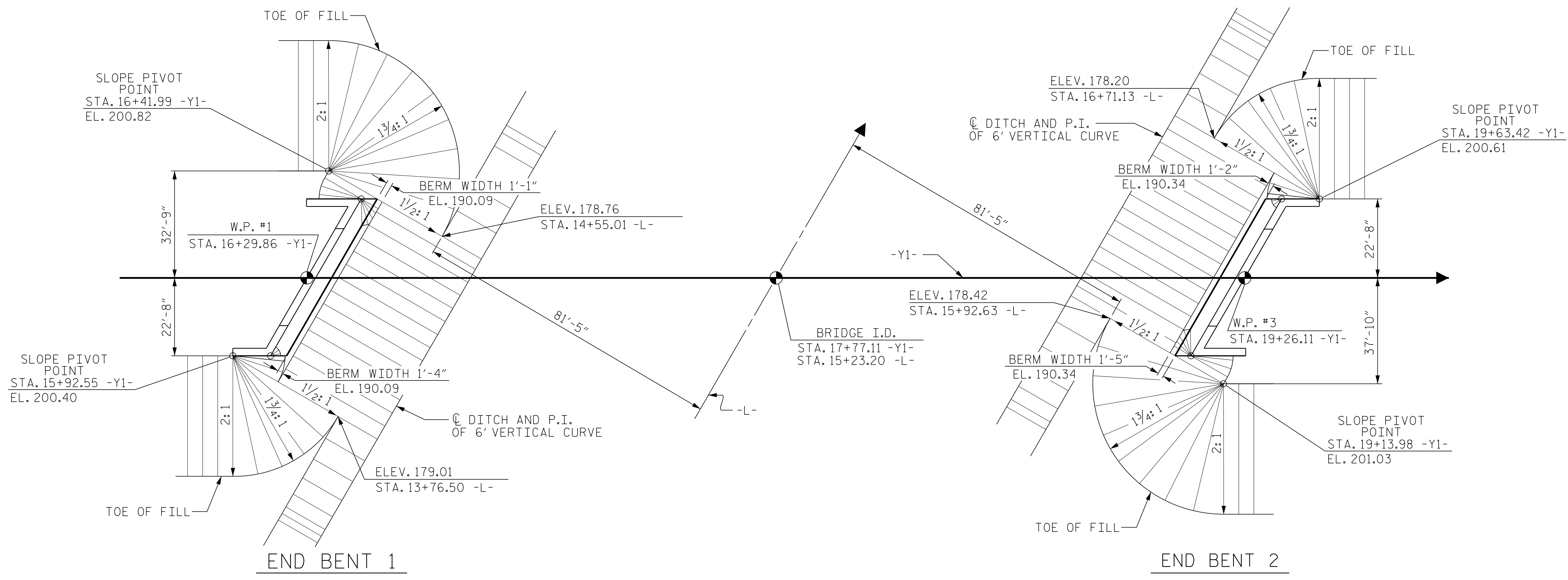
PLAN - GRADING
