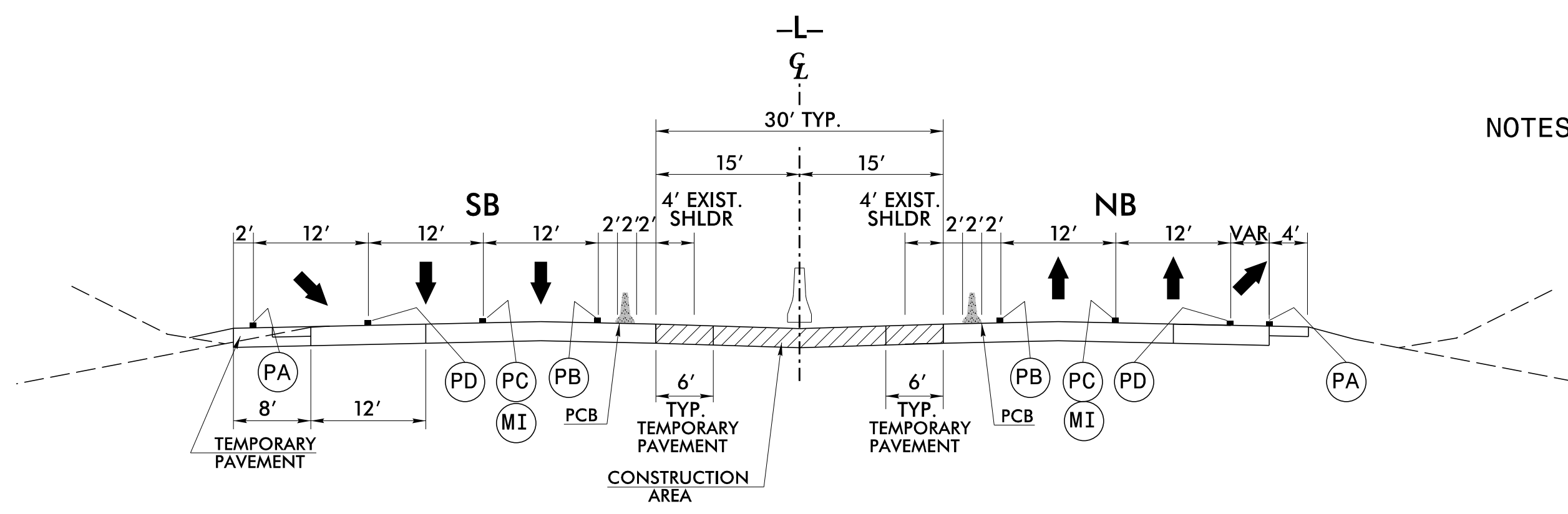
TYPICAL SECTION B-B -L- STA. 145+00 +/-
