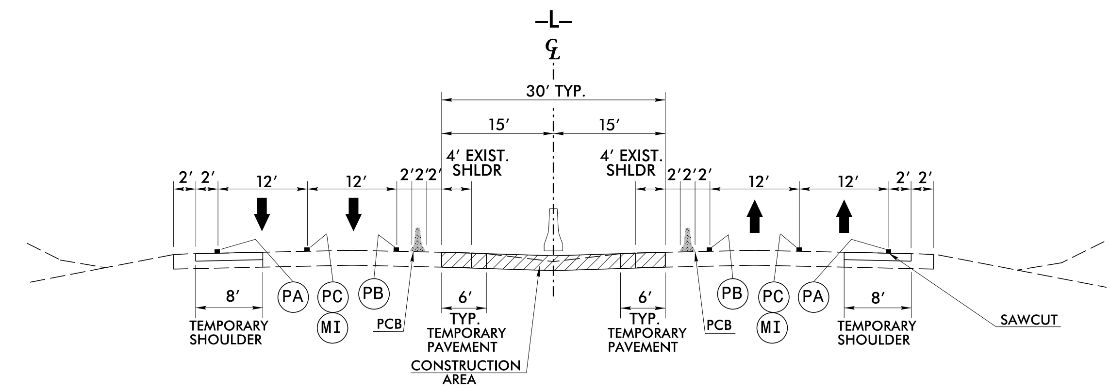
TYPICAL SECTION A-A -L- STA. 150+50 +/-
