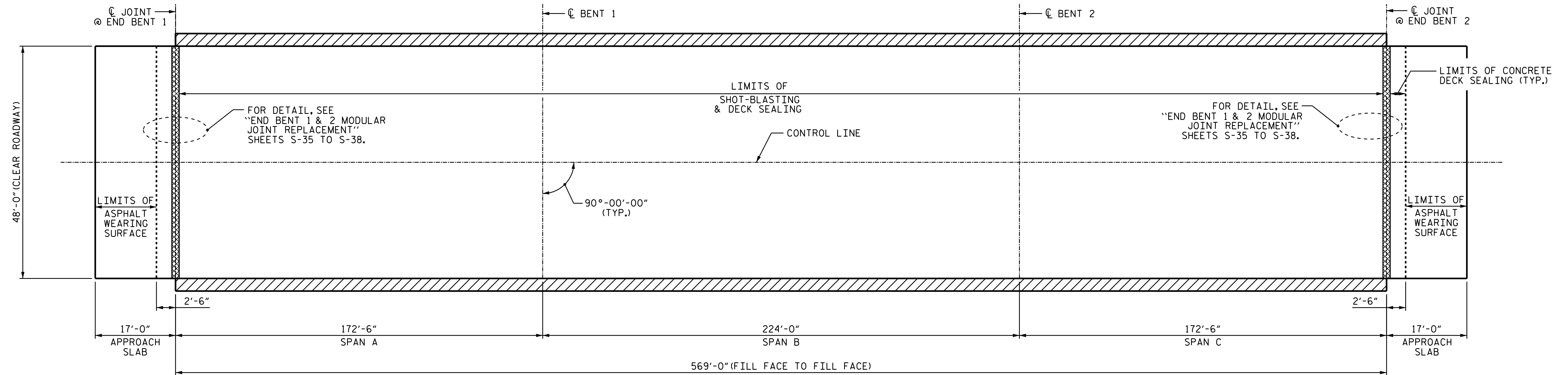
PLAN OF SPANS - DECK REPAIR
