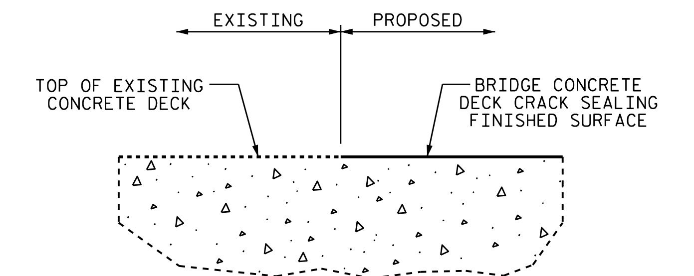
DETAIL OF CONCRETE DECK CRACK SEALING
