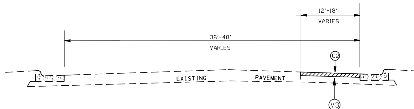
TYPICAL SECTION NO.22 PAVE TOP OF RAMP MAP 15 I-277 OUTER TO COLLEGE ST
