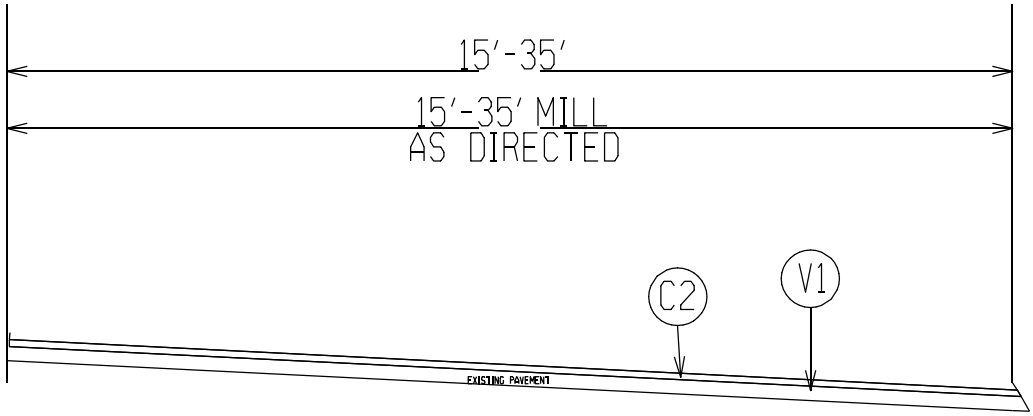
TYPICAL SECTION 2
