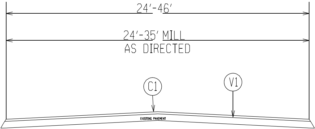
TYPICAL SECTION 1
