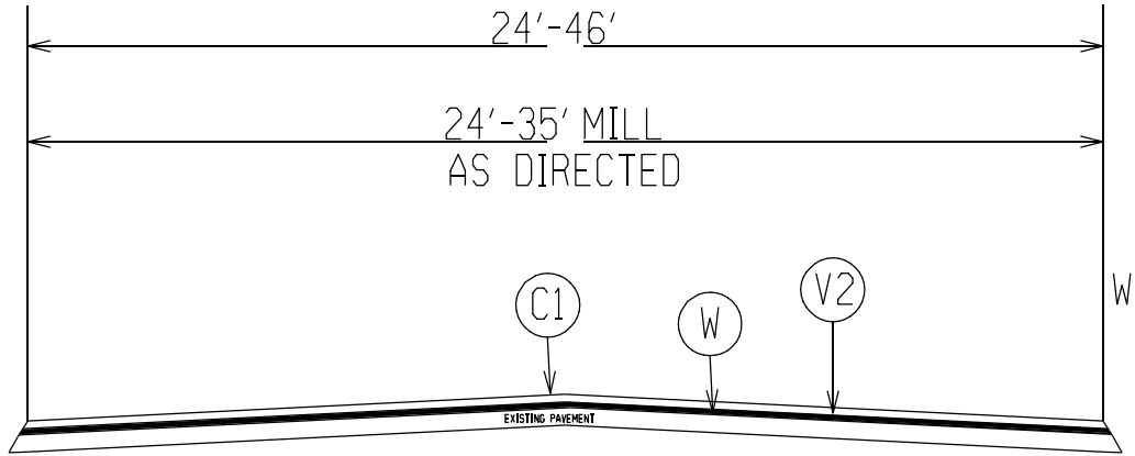
TYPICAL SECTION 3
