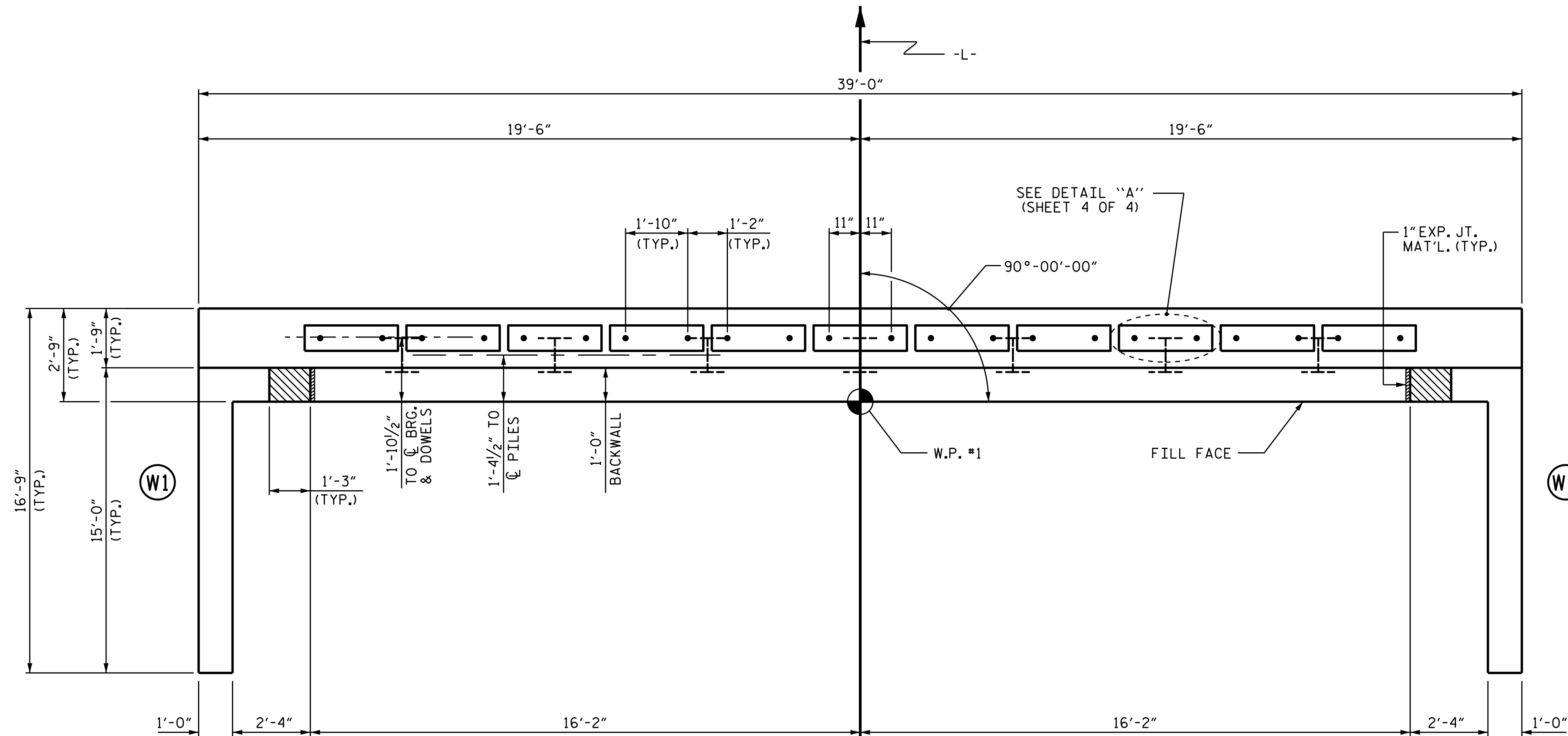
PLAN
