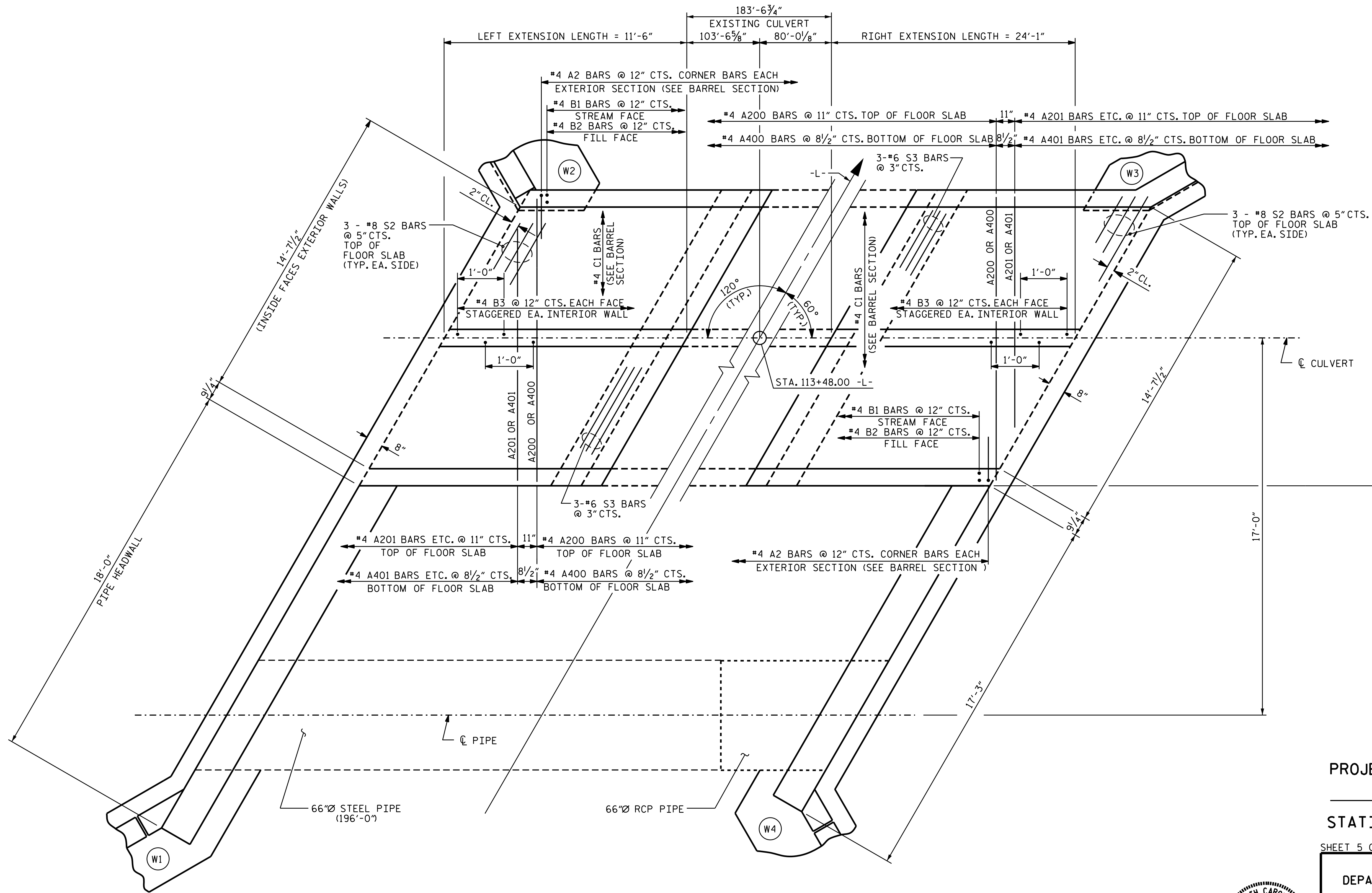
PLAN - FLOOR SLAB
