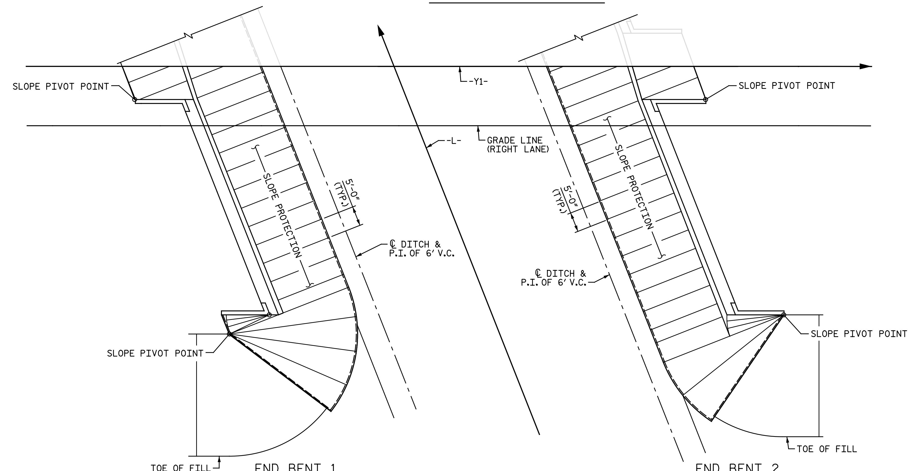
END BENT 1 PLAN - GRADING END BENT 2
