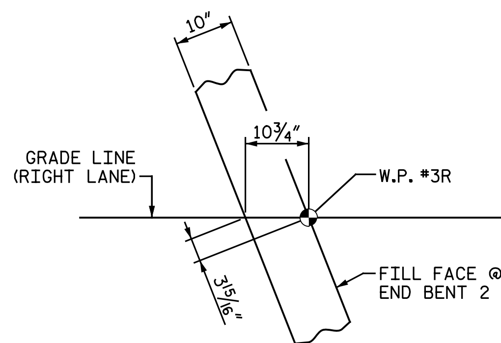
DETAIL "B"
