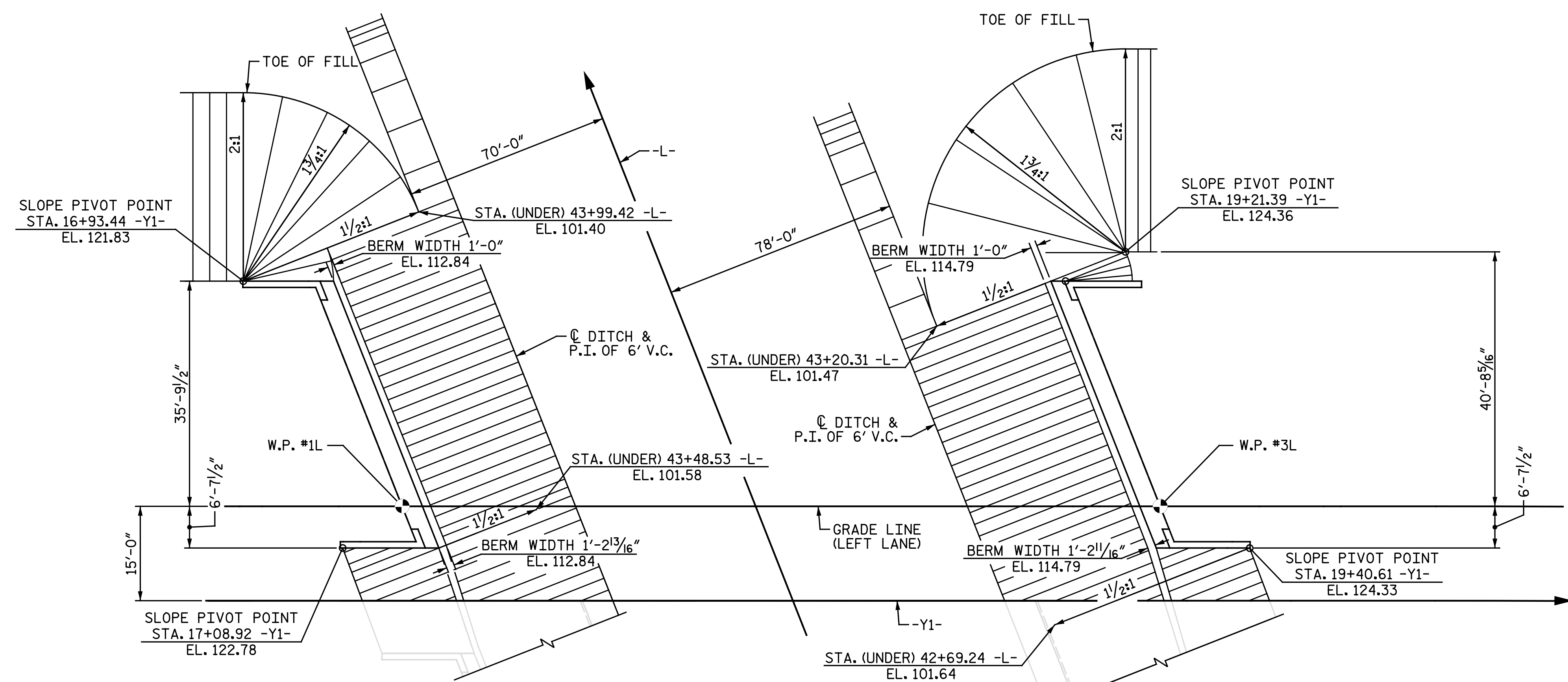
END BENT 1 PLAN - GRADING END BENT 2
