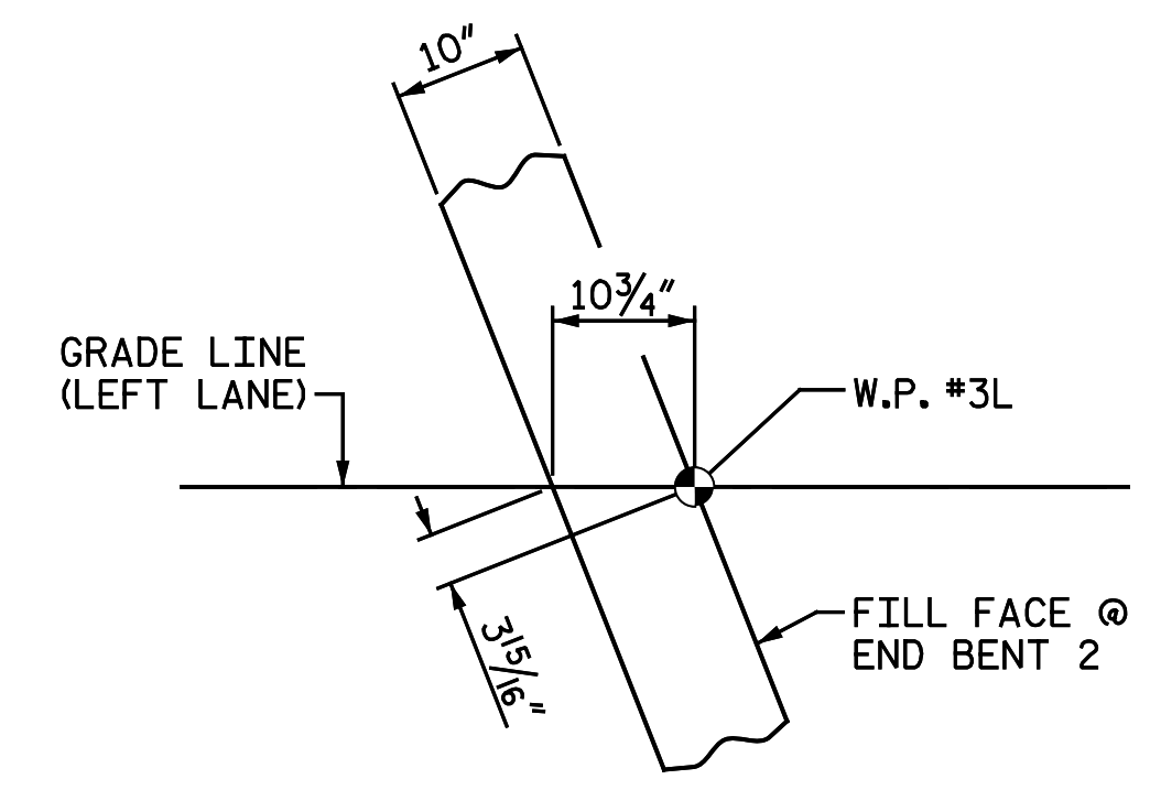
DETAIL "B"
