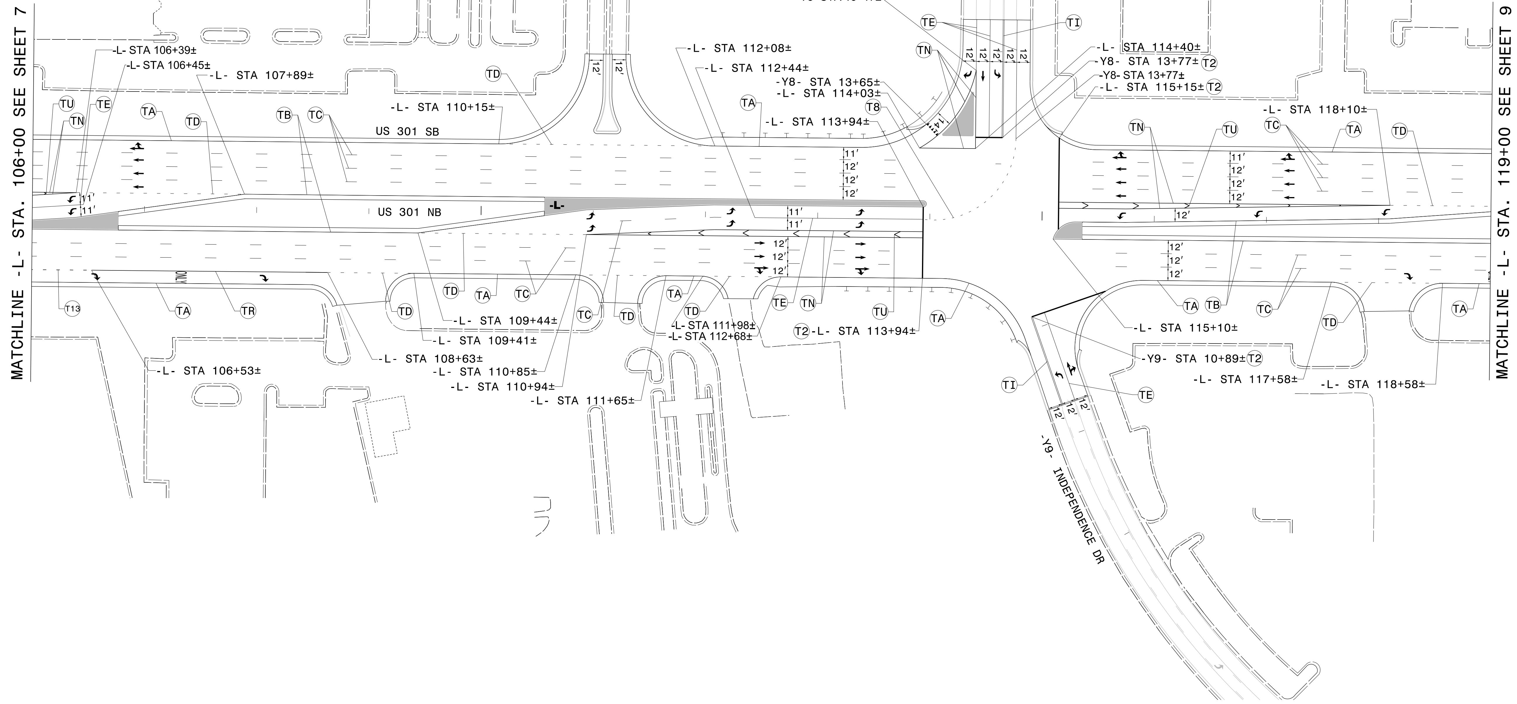
PAVEMENT MARKING DETAIL
