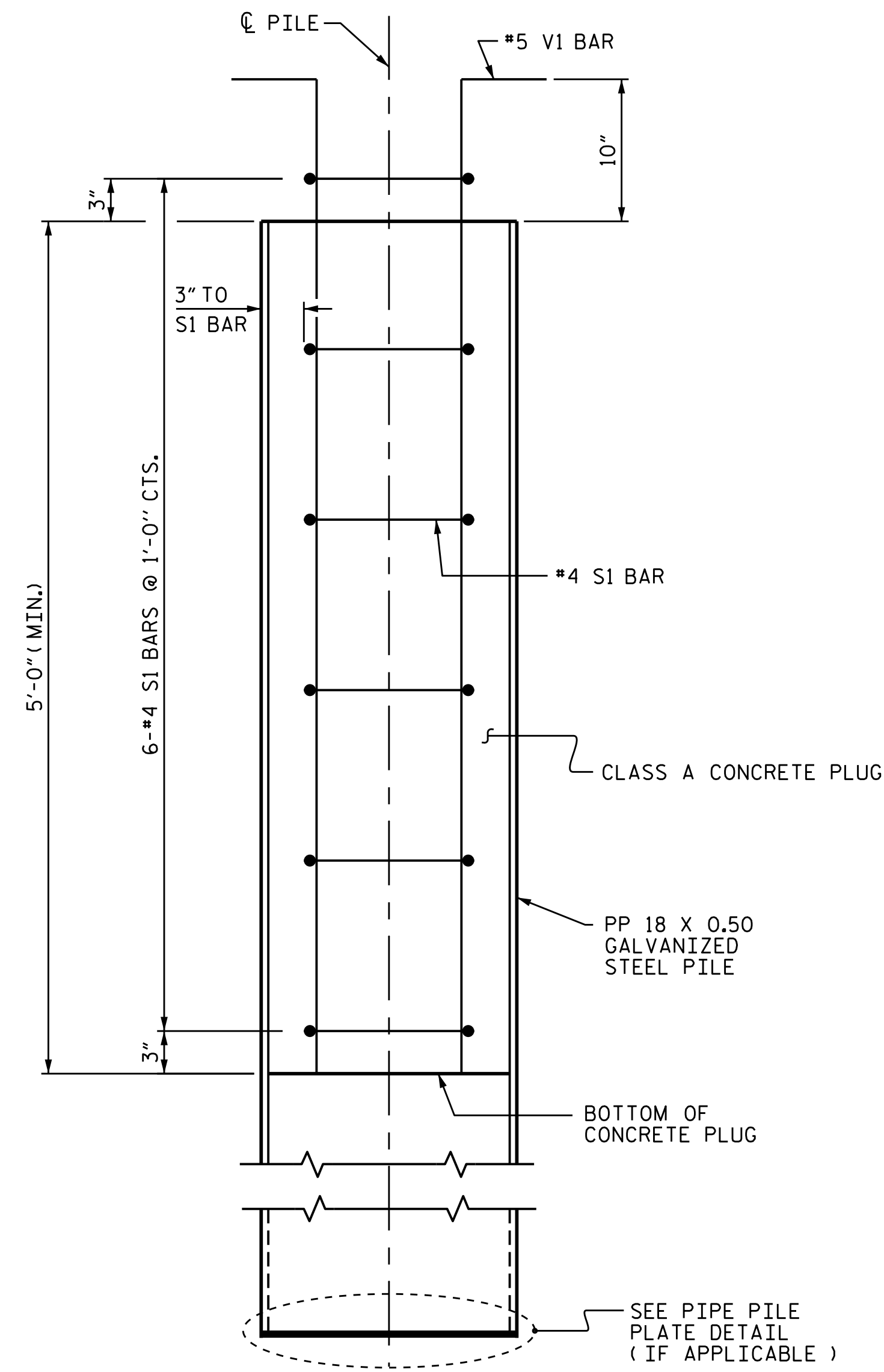
ELEVATION PP 18 X 0.50 GALVANIZED STEEL PILE ( OPEN OR CLOSED END )
