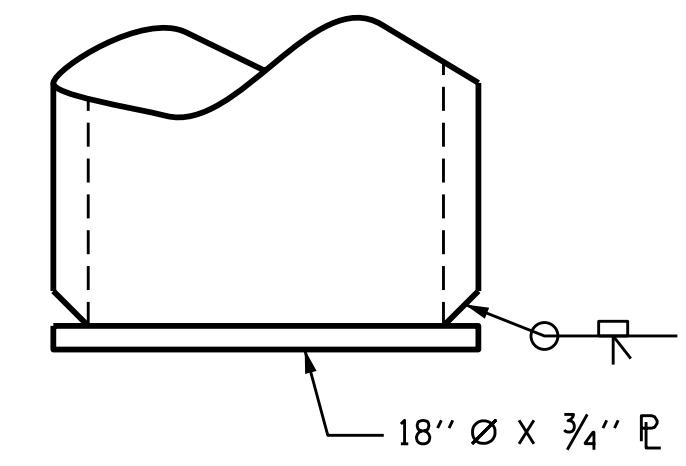
PIPE PILE PLATE DETAIL ( IF APPLICABLE )
