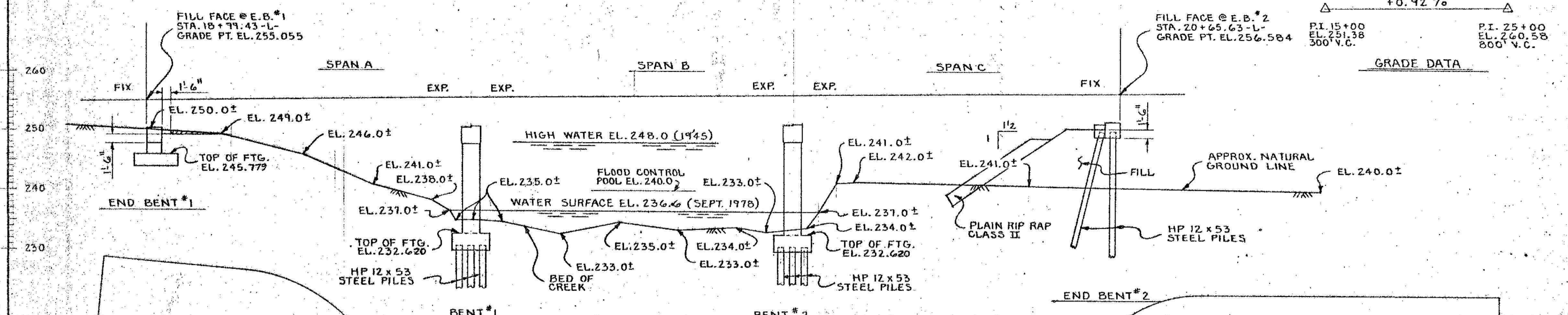
SECTION ALONG & BRIDGE & ROADWAY (LINE-L-) BENTS & END BENTS ON SECTION AT RIGHT ANGLES TO BENTS.
