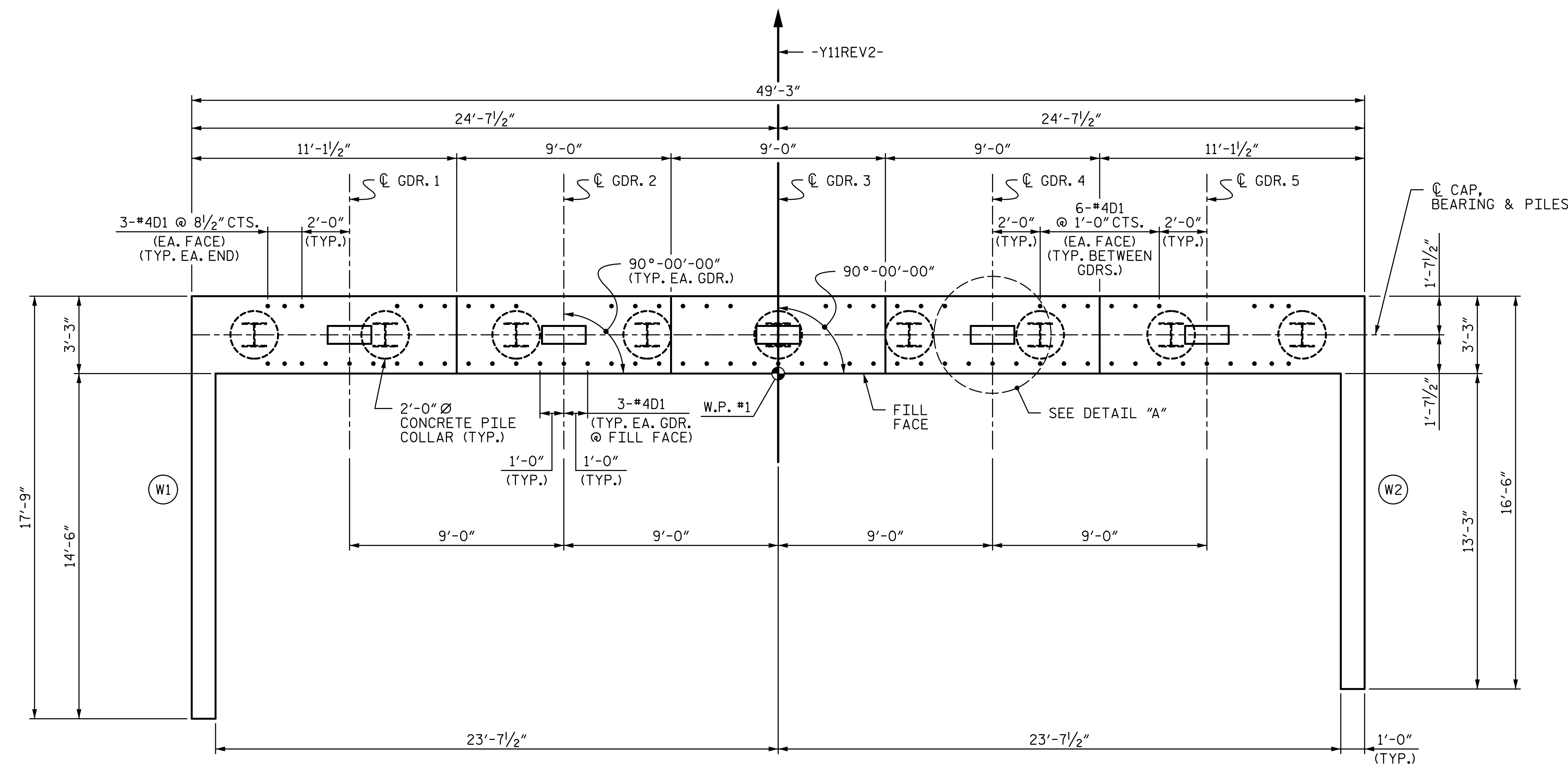
PLAN
