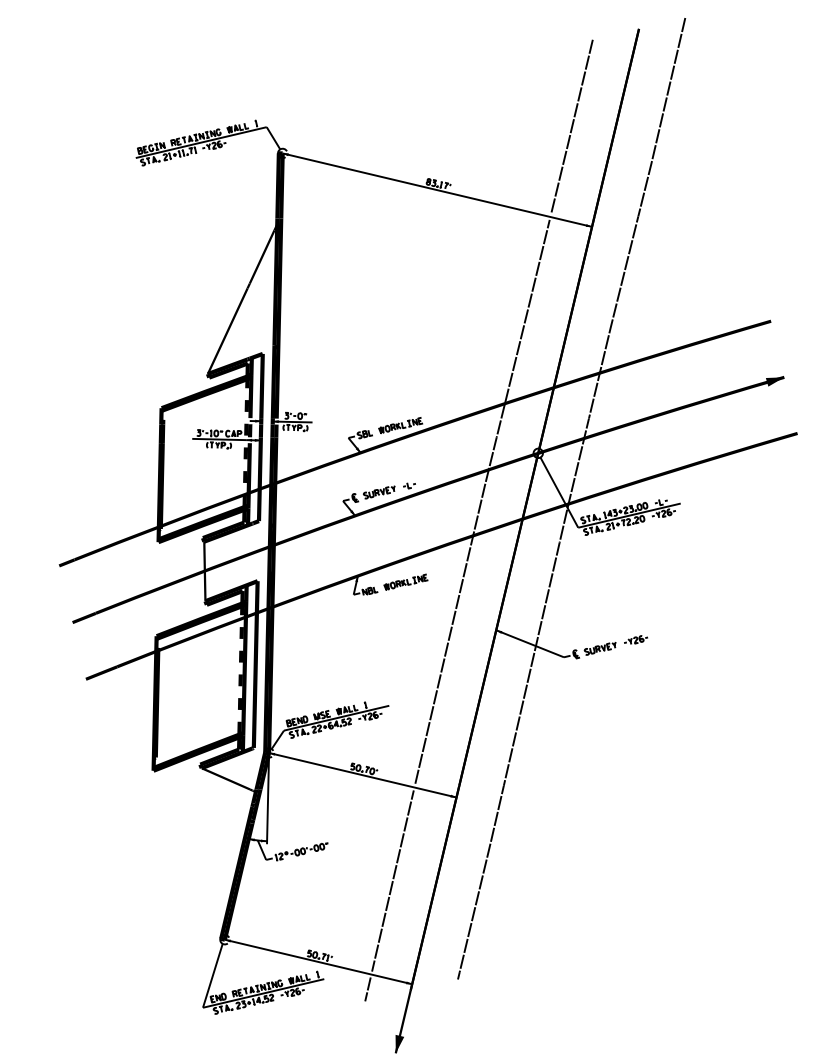
RETAINING WALL NO. 1 PLAN VIEW
