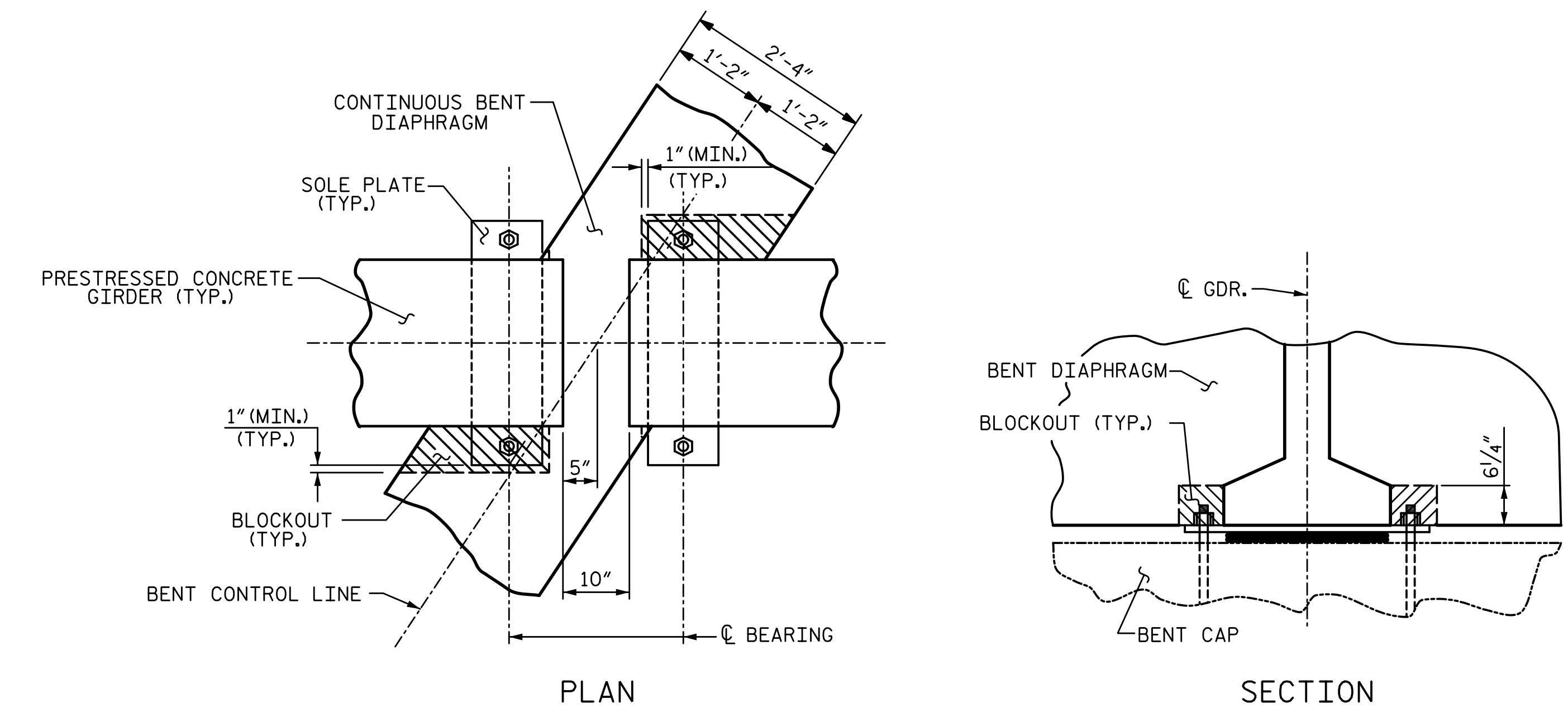
CONTINUOUS BENT DIAPHRAGM BLOCK-OUT DETAIL
