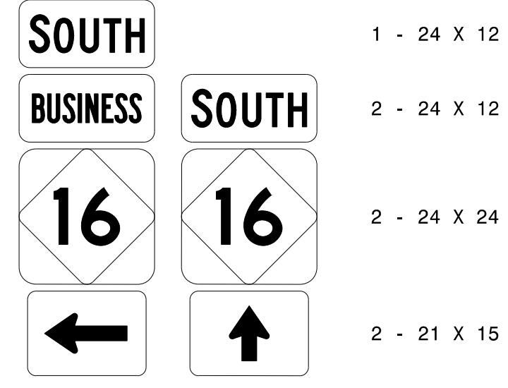
MOUNT BELOW SIGN 306 IN 1 INSTALLATION
