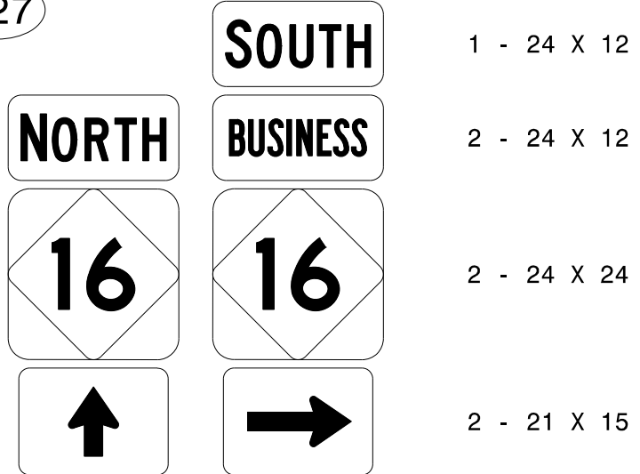
TWO "U" POSTS PER SIGN
