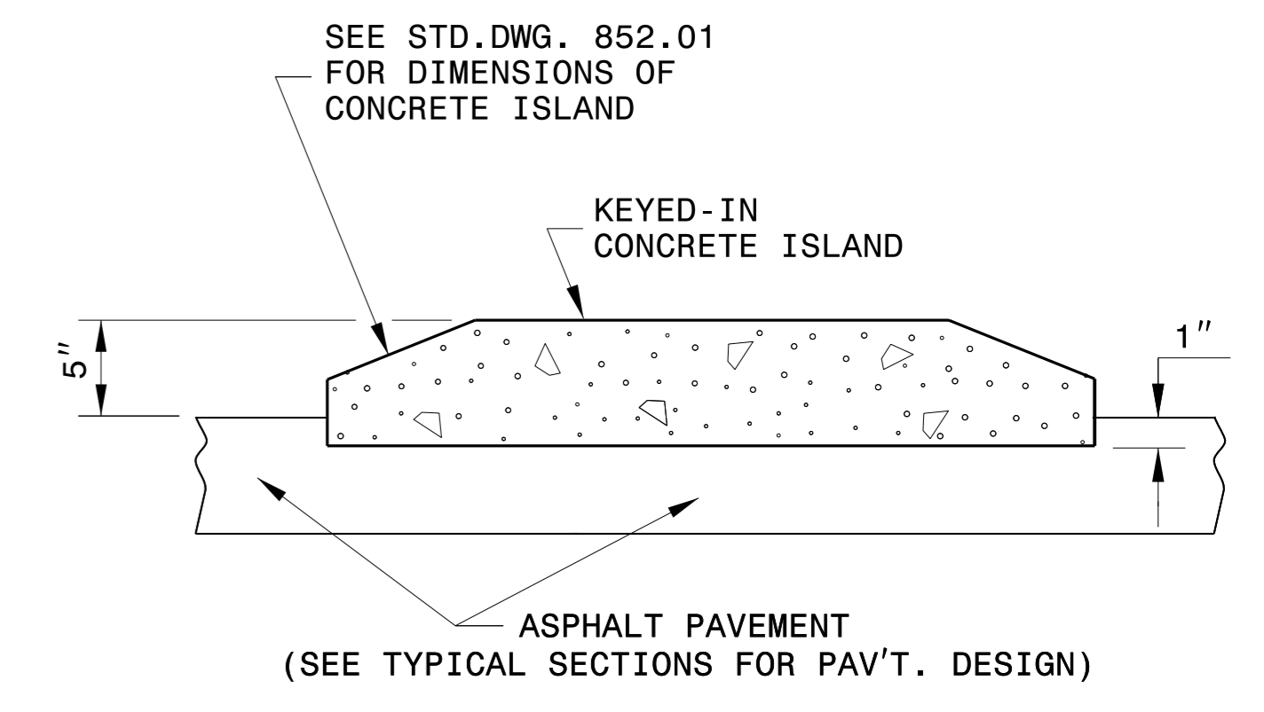
SECTION C-C
