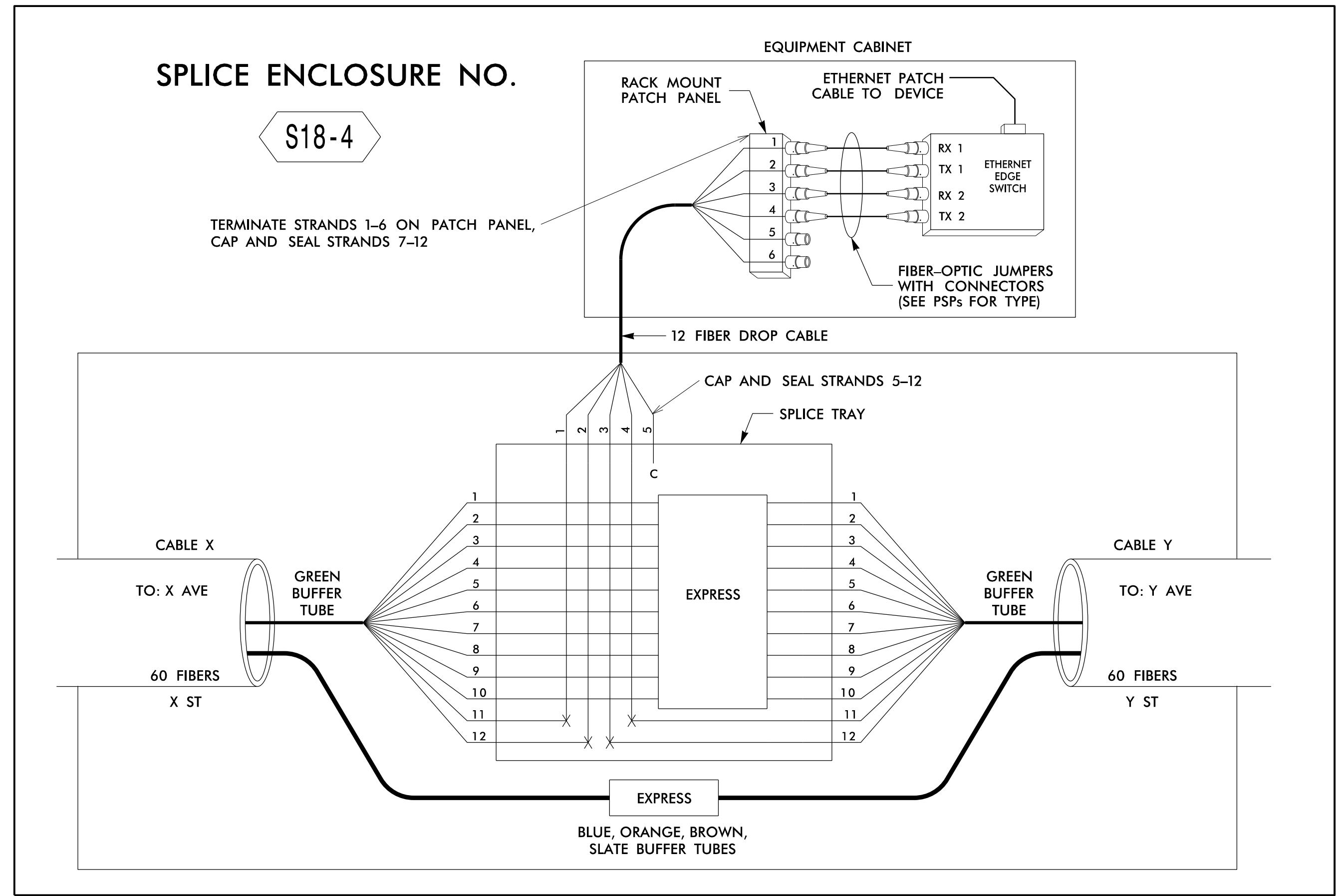
SPLICE ENCLOSURE NO. S18-4
