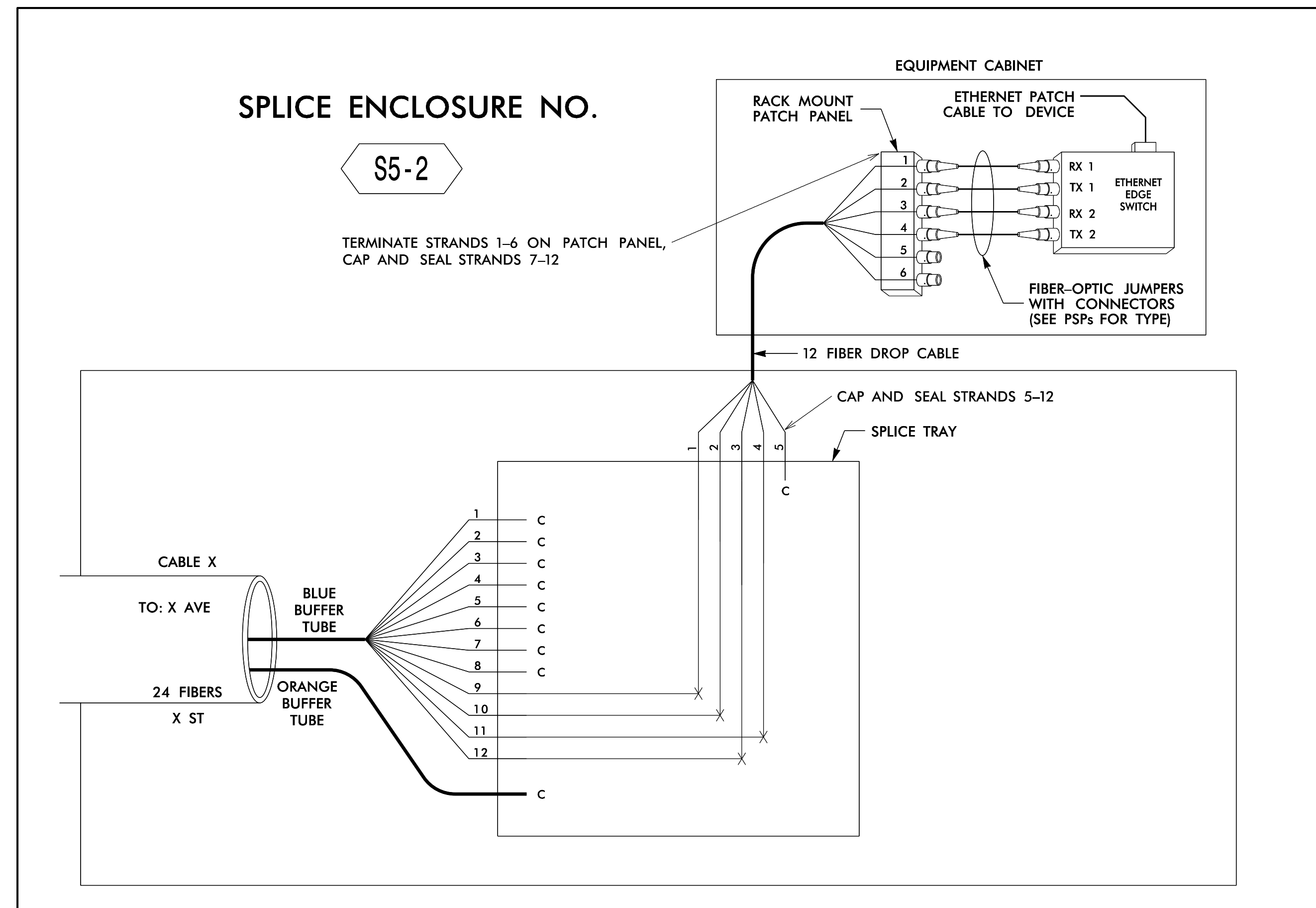
SPLICE ENCLOSURE NO. S5-2
