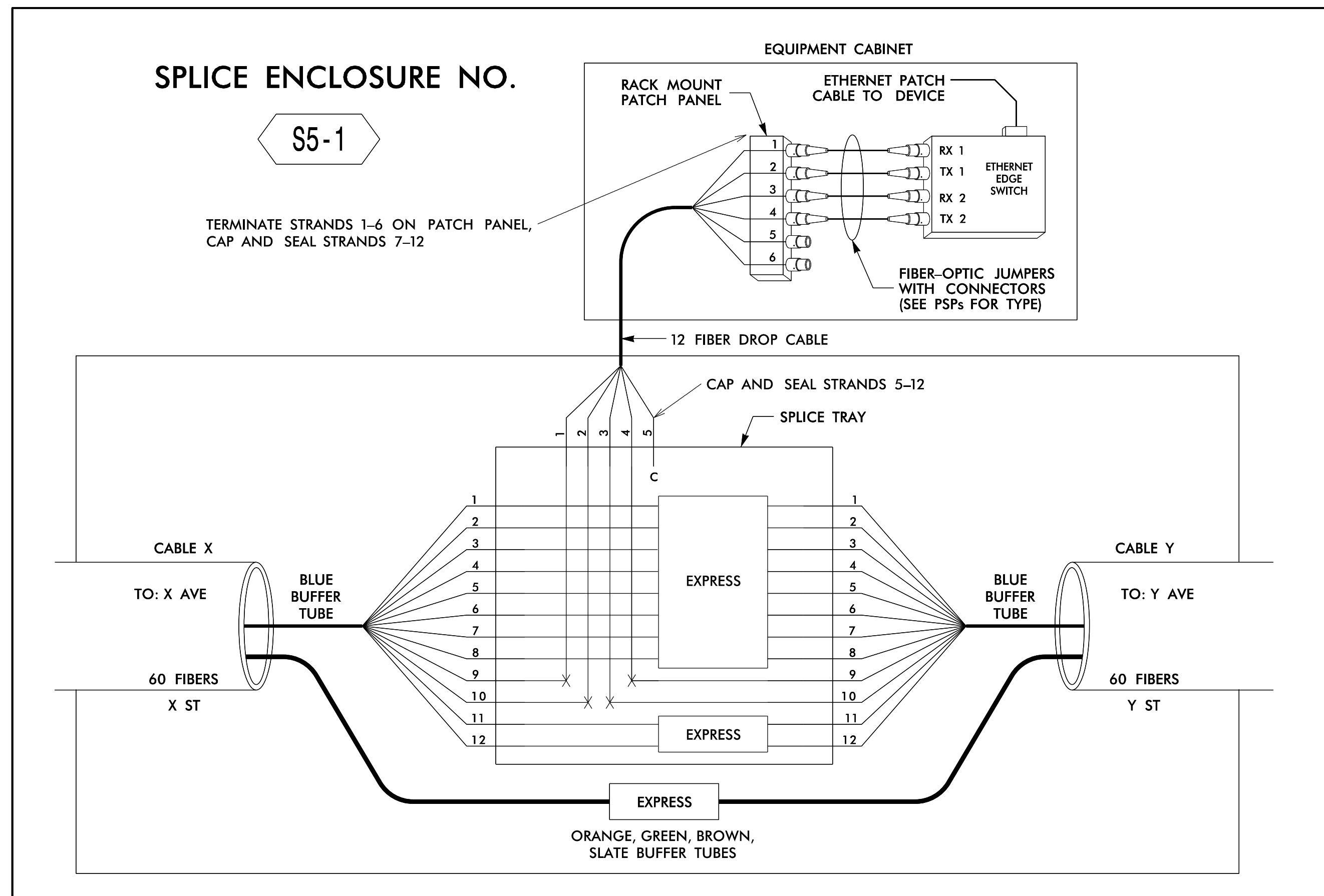
SPLICE ENCLOSURE NO. S5-1
