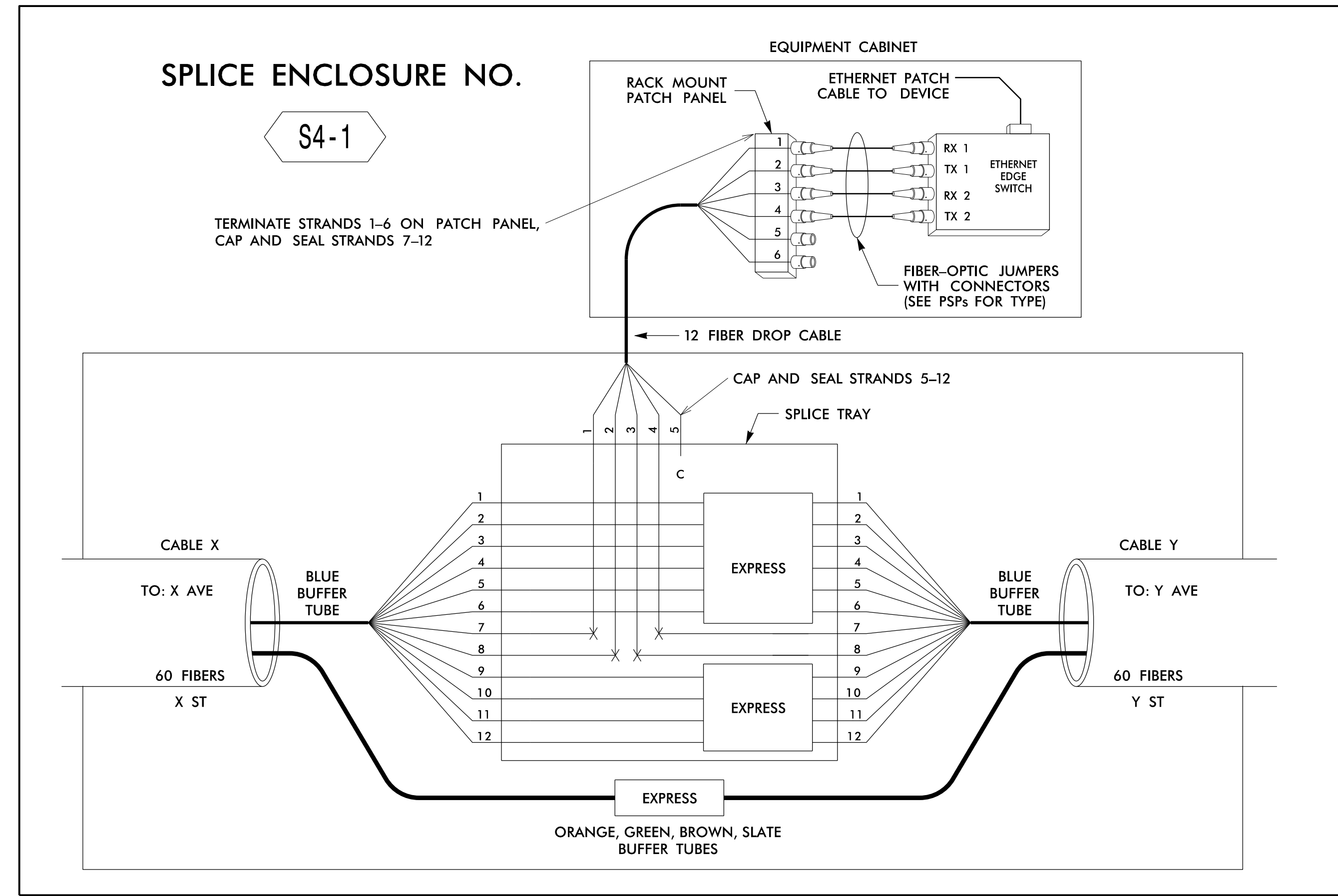
SPLICE ENCLOSURE NO. S4-1
