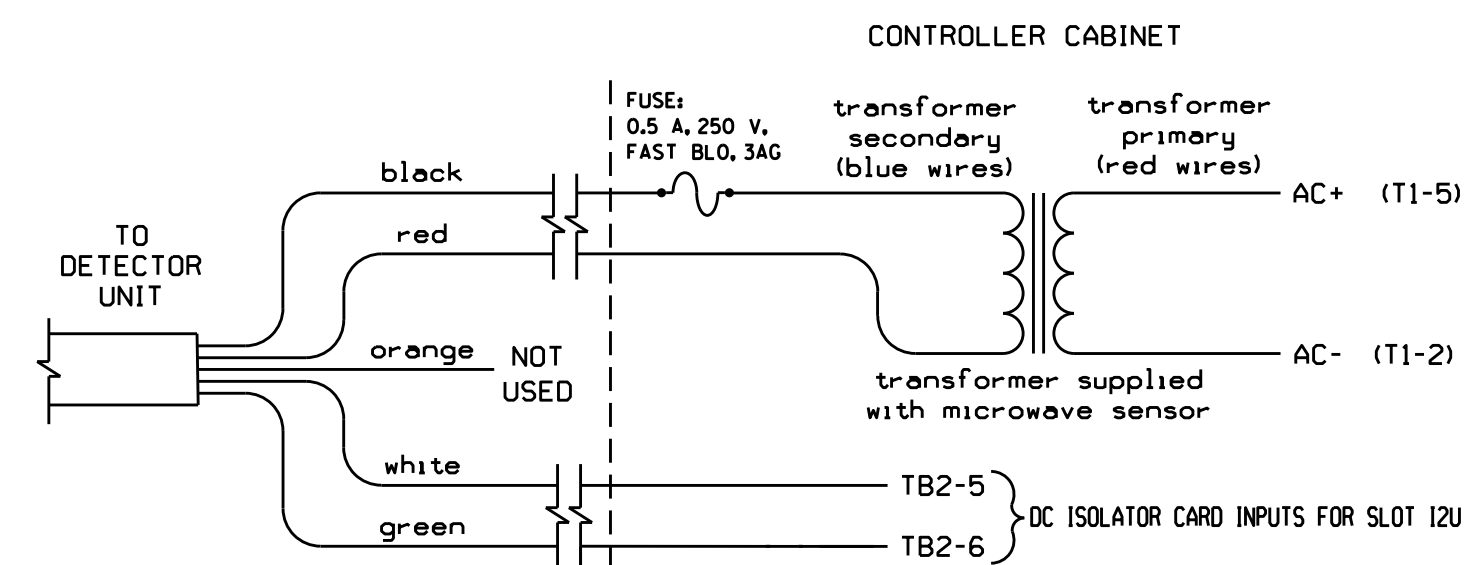
TYPICAL WIRE LIST
