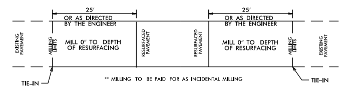
PAVEMENT TIE-IN DETAIL
