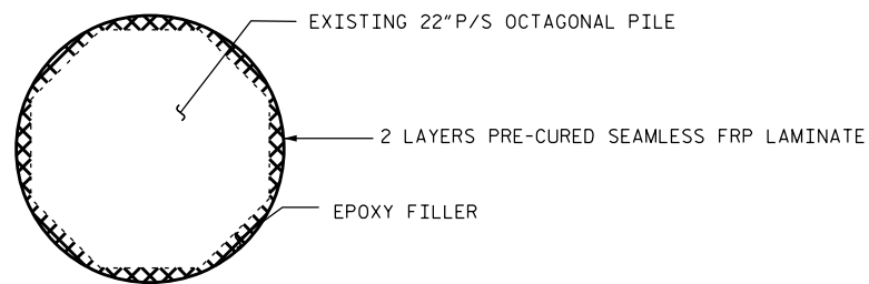
PILE SECTION DETAIL
