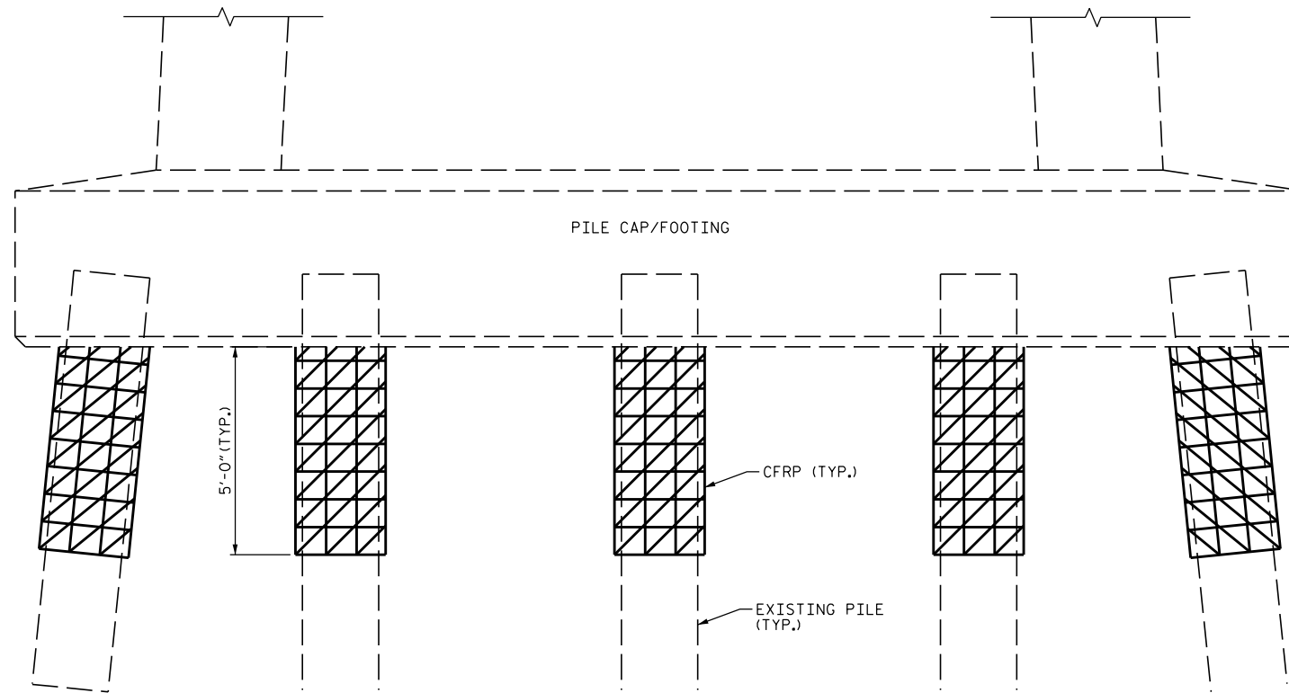
TYPICAL FOOTING SHOWN - ELEVATION
