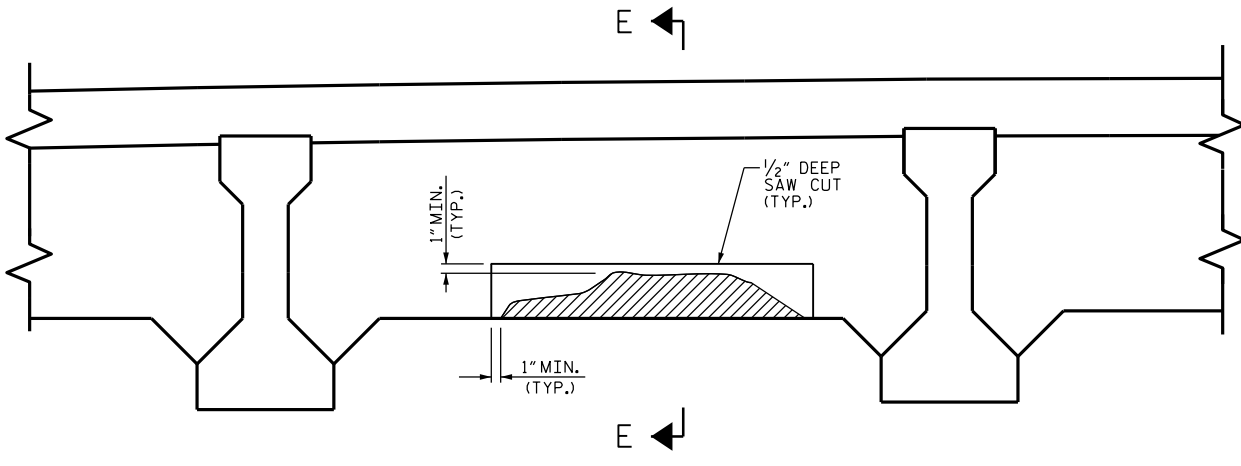
TYPICAL SECTION
