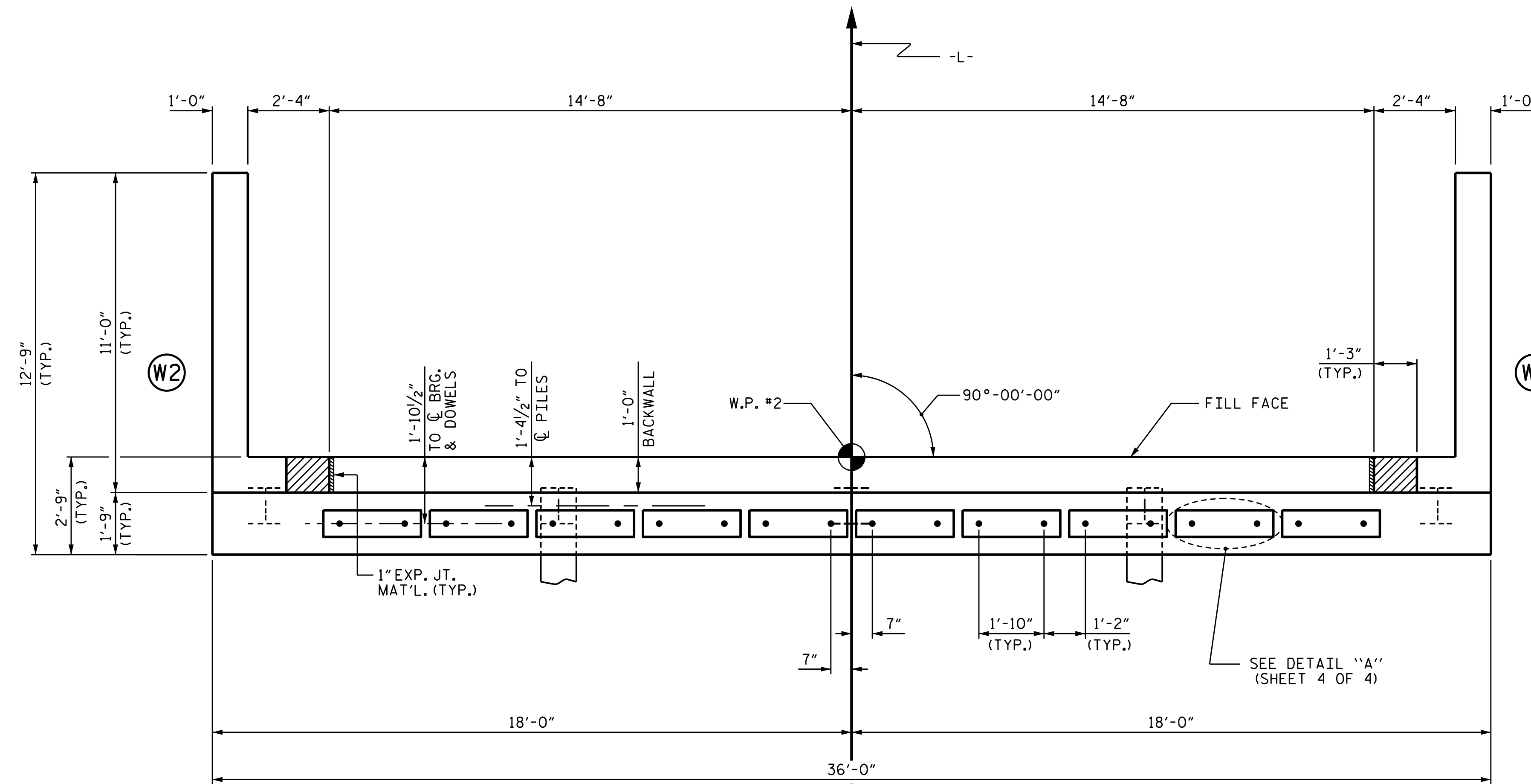
PLAN
