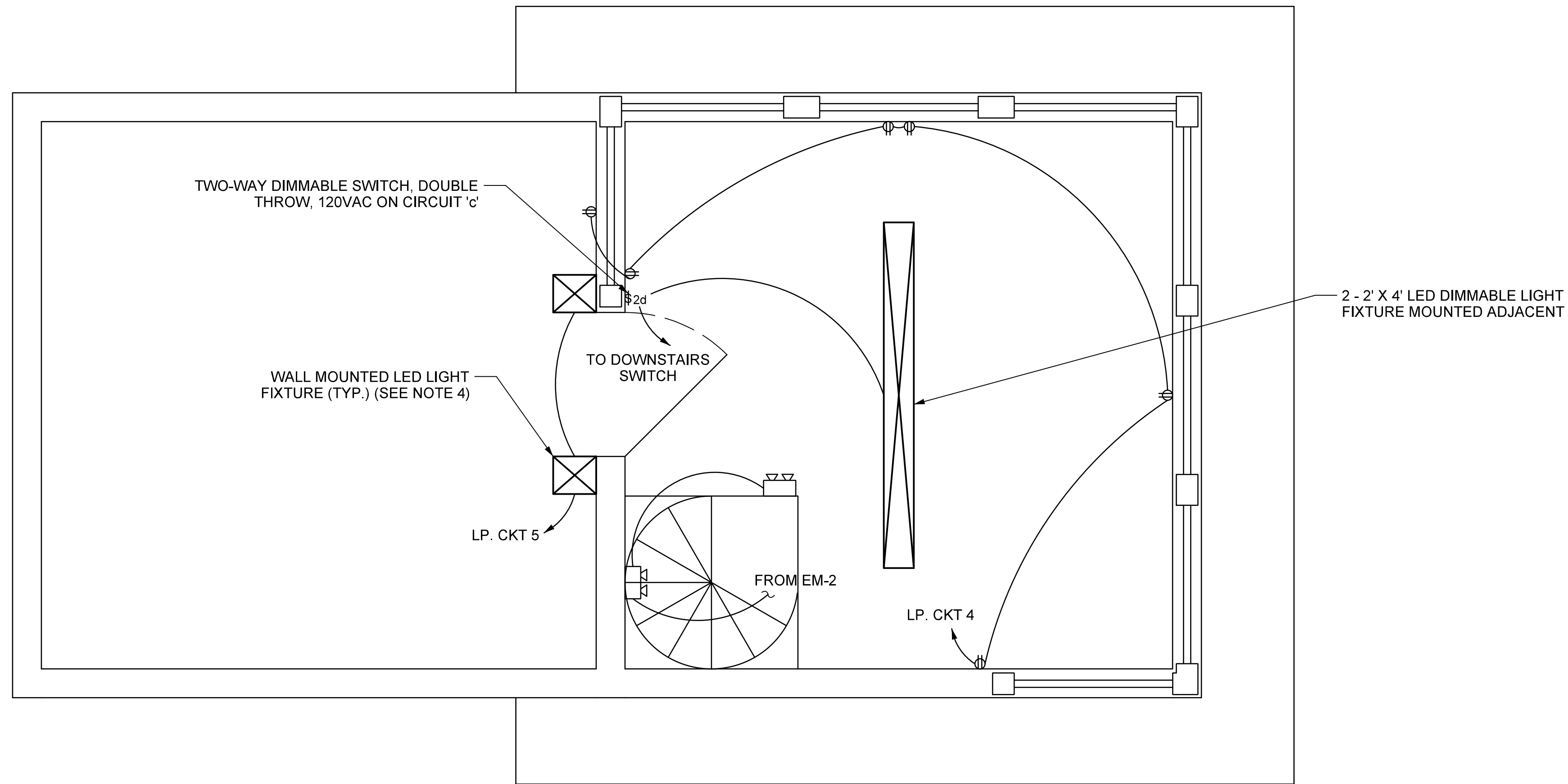
SECOND FLOOR LAYOUT SCALE: 1/2" = 1'-0"
