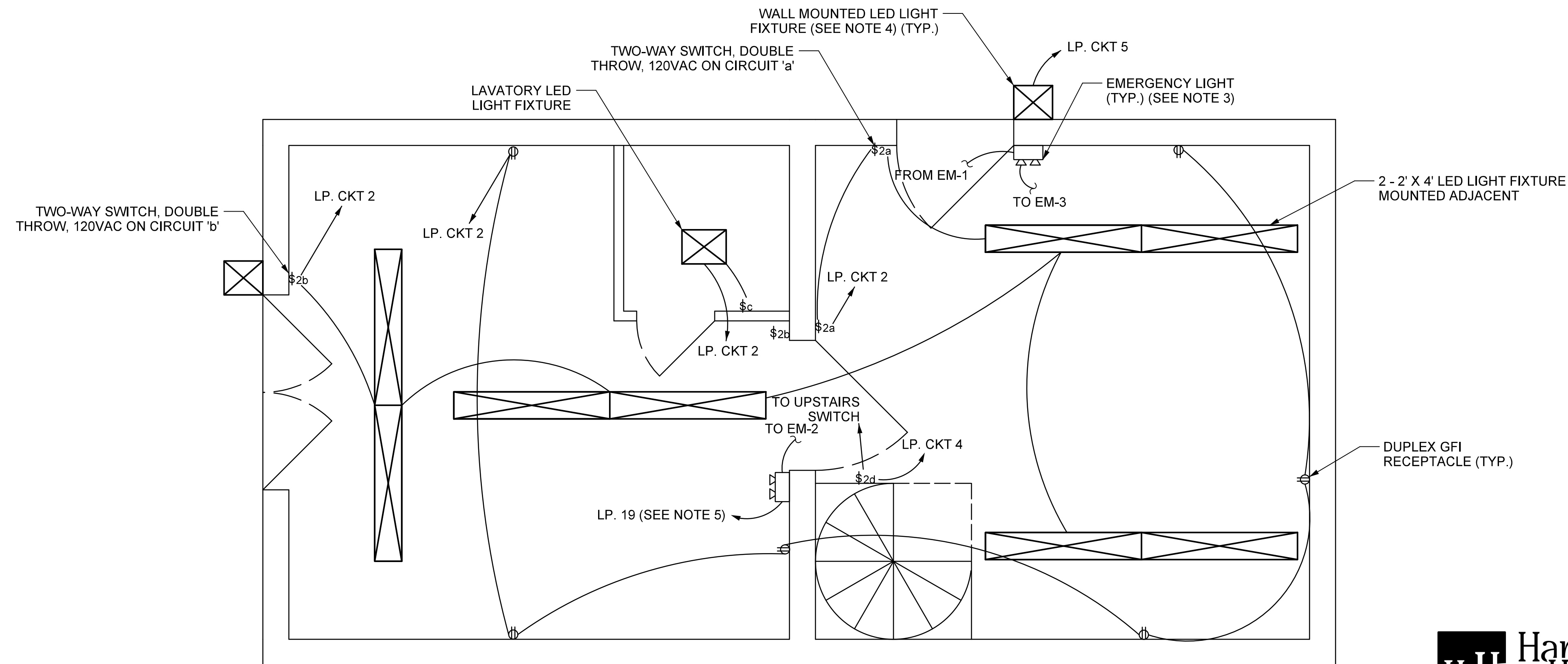
FIRST FLOOR LAYOUT SCALE: 1/2" = 1'-0"
