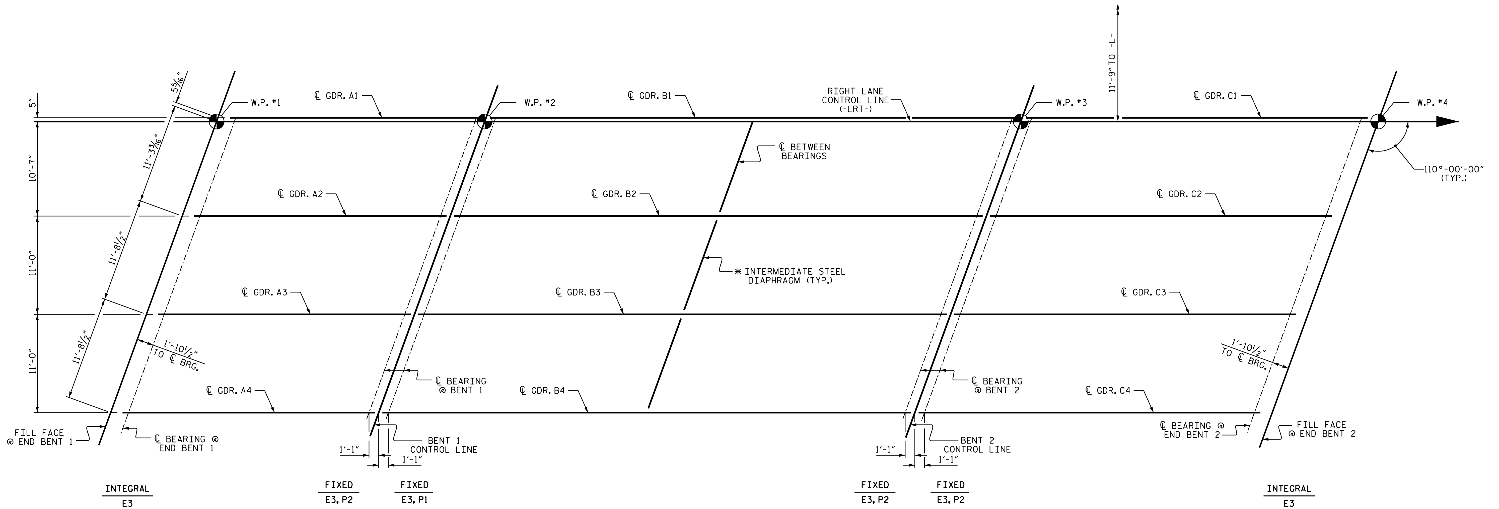
GIRDER LAYOUT * SEE "INTERMEDIATE STEEL DIAPHRAGMS FOR TYPE III PRESTRESSED CONCRETE GIRDERS".
