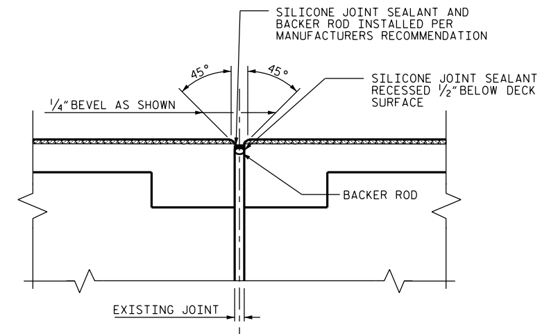
PROPOSED JOINT
