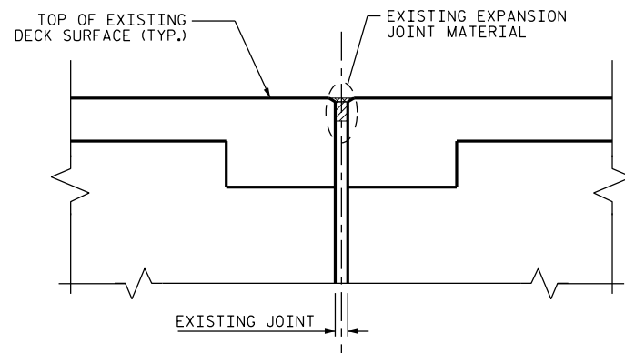
EXISTING
