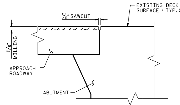
MINIMUM EXISTING JOINT DEMOLITION
