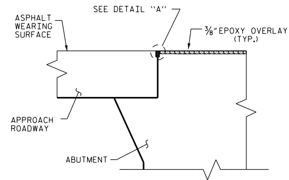
PROPOSED JOINT
