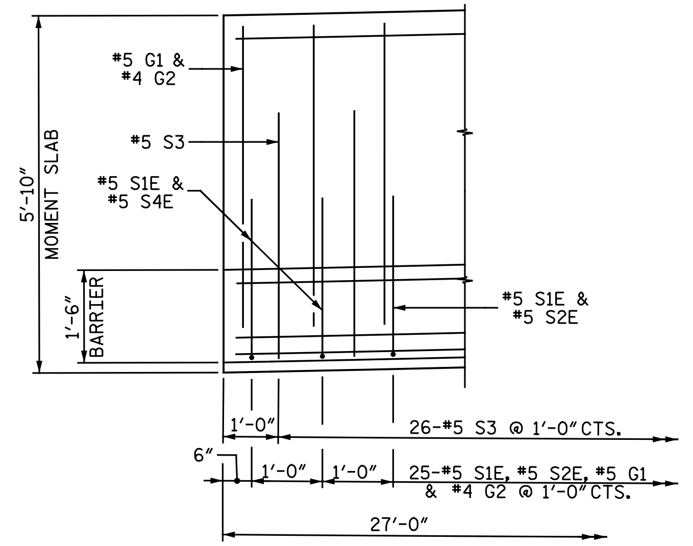
DETAIL "B"
