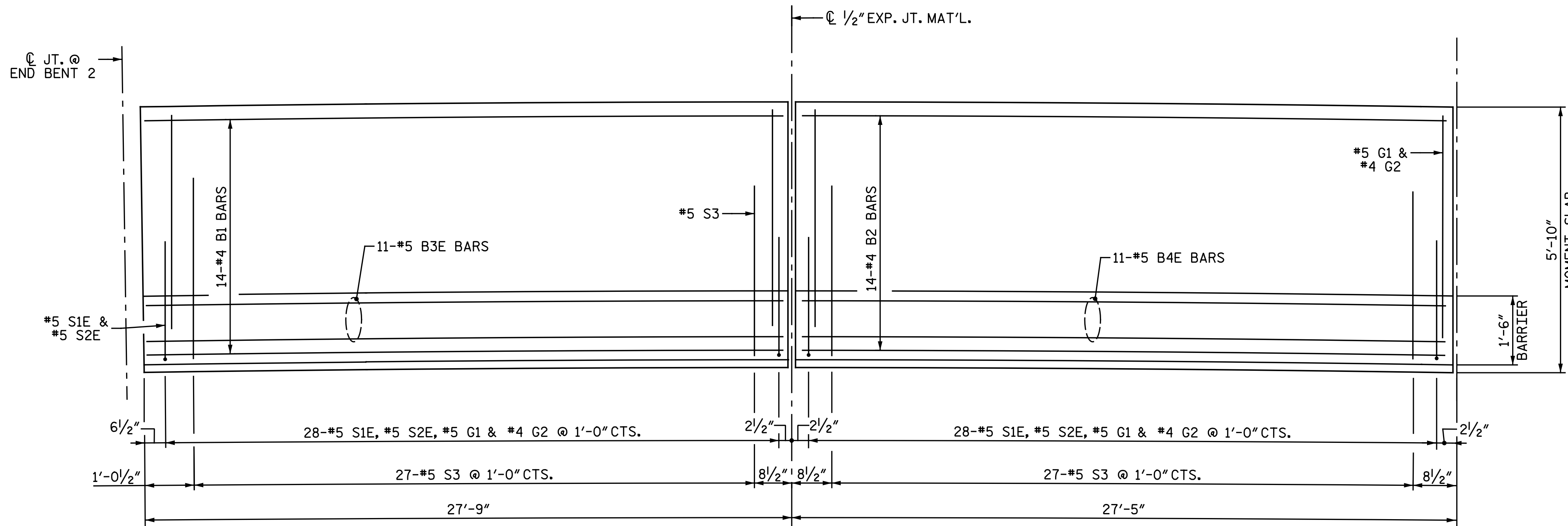
DETAIL "A"
