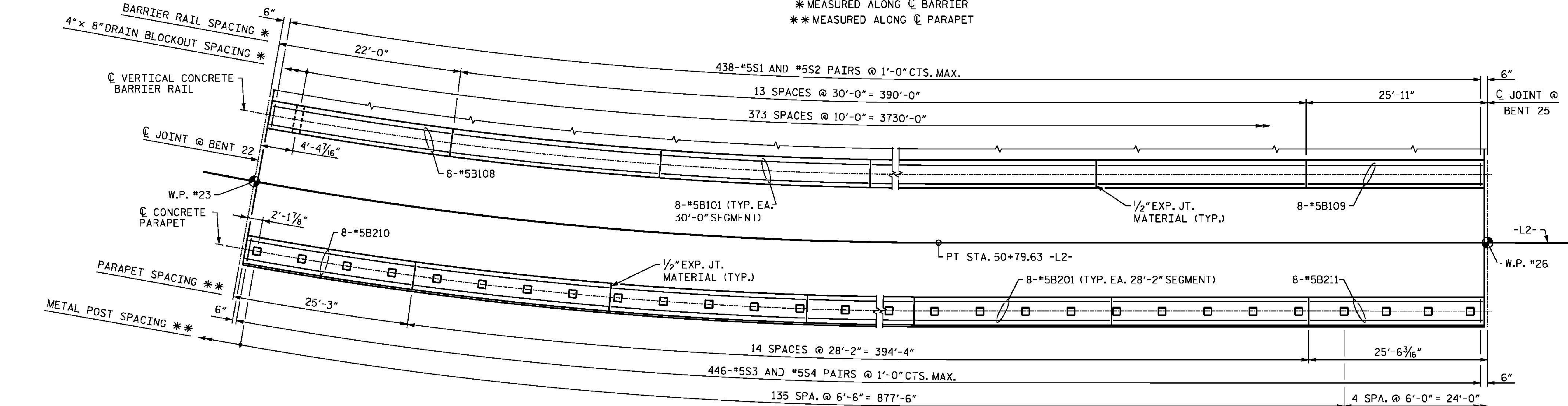
PLAN - UNIT 8 * MEASURED ALONG C BARRIER ** MEASURED ALONG C PARAPET
