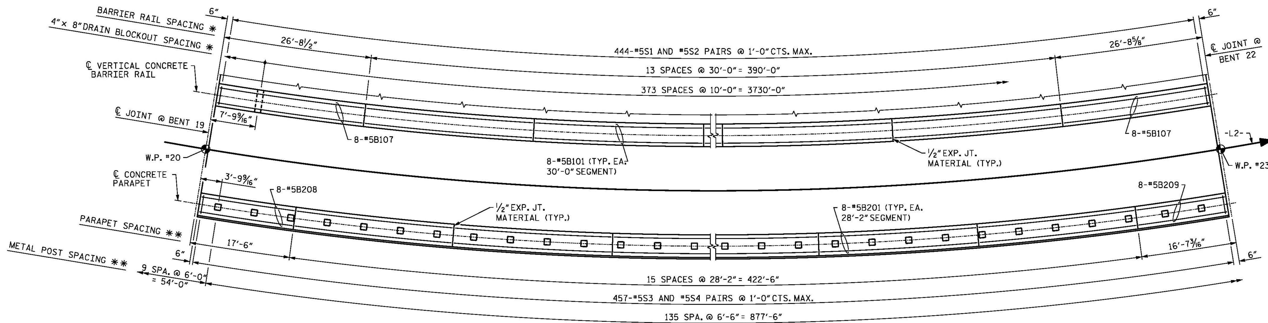
PLAN - UNIT 7 * MEASURED ALONG C BARRIER ** MEASURED ALONG C PARAPET
